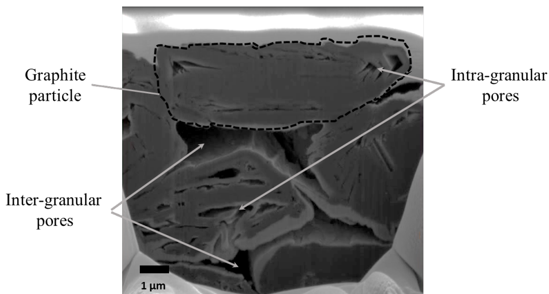
Figure 5 : SEM image showing the section of the pristine composite negative electrode. The cross section was realized by Focused Ion Beam (FIB).
