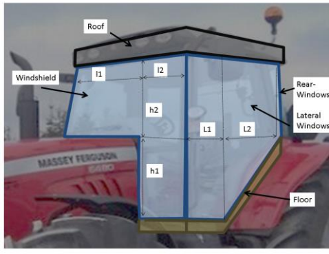
Figure 4. Schematic design of the tractor cabin and dimensions (m 2 ): A_{\text{front}}=1.70 , A_{\text{rear}}=1.46 , A_{\text{lat}}=1.73 , A_{\text{roof}}=2.1 , A_{\text{base}}=2.86
