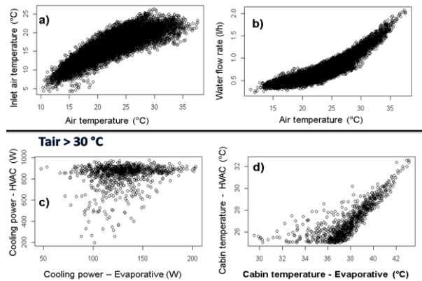
Figure 8. In the upper part, a) - air inlet temperature and b) water consumption of the adiabatic system according to ambient air temperature for common situations – In the lower part, c) cooling power of the conventional HVAC versus adiabatic system in critical situations, d) cabin temperature with HVAC versus adiabatic system in critical situations
