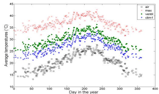
Figure 7. Cabin temperature averages in hot diurnal situations for each day under various climates and related average of air temperature
