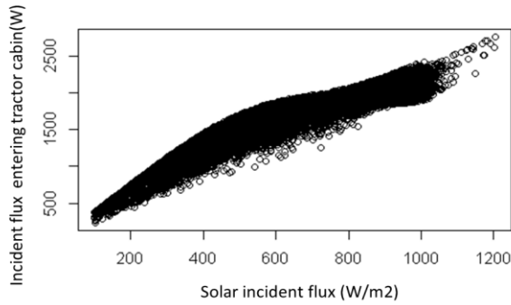
Figure 5. Solar income entering the cabin (W) versus solar incident radiation ( \text{W/m}^2 )
