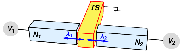
FIG. 1. Schematic view of the setup: a grounded TS nanowire is tunnel coupled (with hopping amplitudes \lambda_1 , \lambda_2 ) to two normal-conducting ( N_1 , N_2 ) leads which are biased at voltages V_1 and V_2 , respectively.
