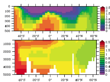
MEDUSA 2, GA-02
