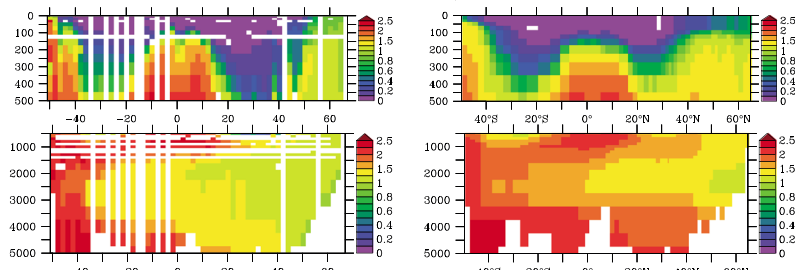
BLING, GA-02
