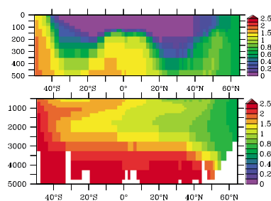
TOPAZ, GA-02
