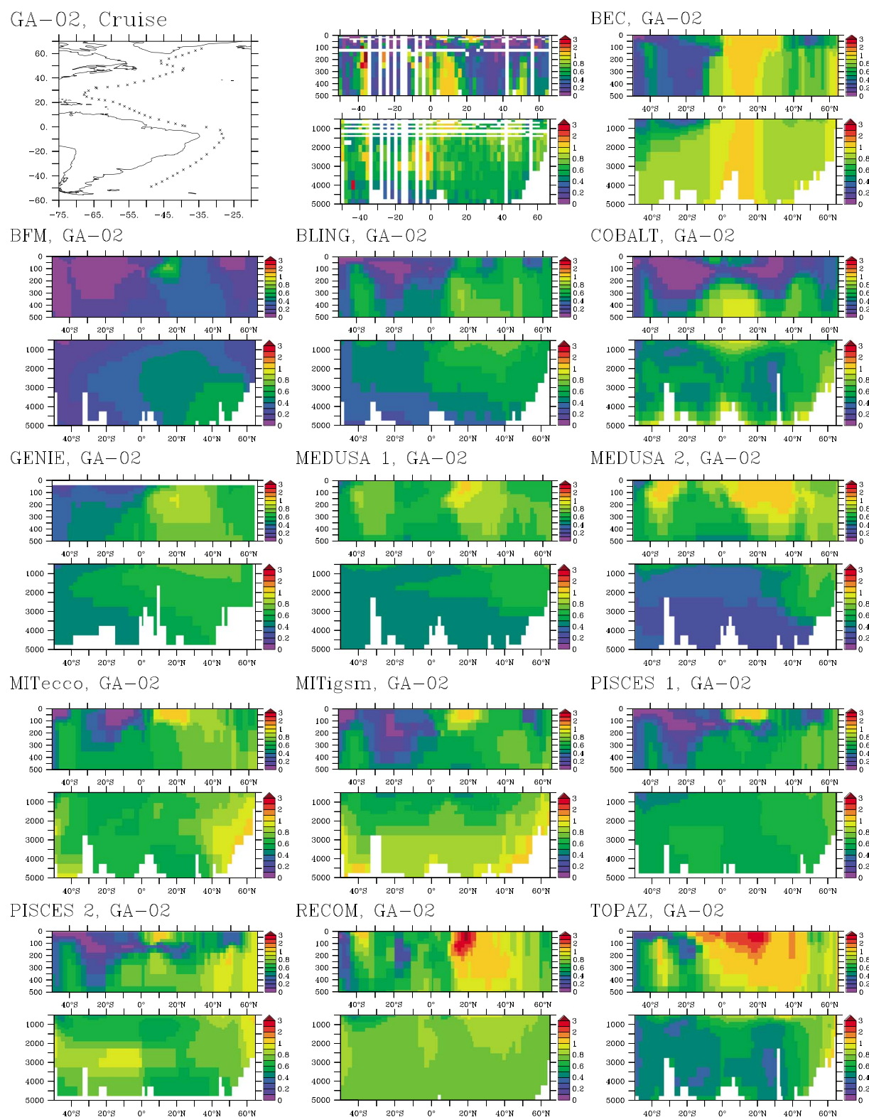
Figure 4. DFe concentrations (nM) from the GA-02 [Rijkenberg et al., 2014] cruise and extracted from the FeMIP models.
