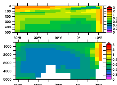
Figure 6. DFe concentrations (nM) from the CoFeMUG cruise [Noble et al., 2012] and extracted from the FeMIP models.
