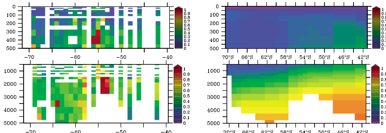
BLING, GIPY-5
