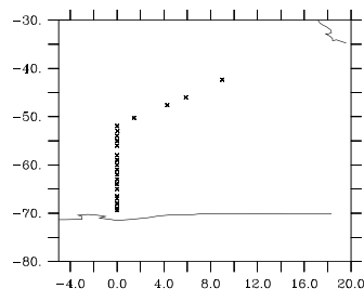
BFM, GIPY-5
