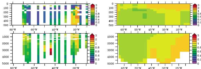
BLING, GA-03
