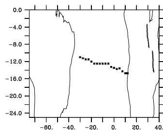
BFM, CoFeMUG
