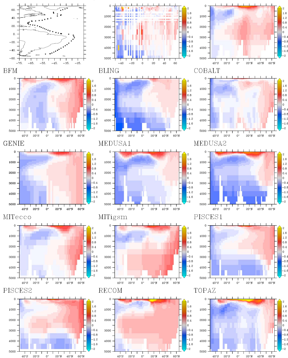
Figure 11. \text{Fe}^* ( \text{Fe}-\text{NO}_3 \times r_{\text{Fe/N}} , nM) from the GA-02 cruise [Rijkenberg et al., 2014] and extracted from the FeMIP models. For models that do not provide \text{NO}_3 , \text{PO}_4 is used and converted to \text{NO}_3 assuming a ratio of 16:1.
