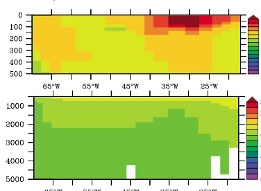
RECOM, GA-03
