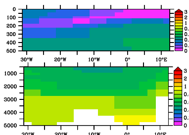
RECOM, CoFeMUG
