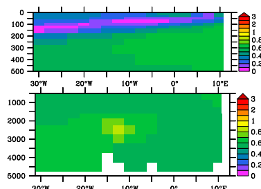
TOPAZ, CoFeMUG
