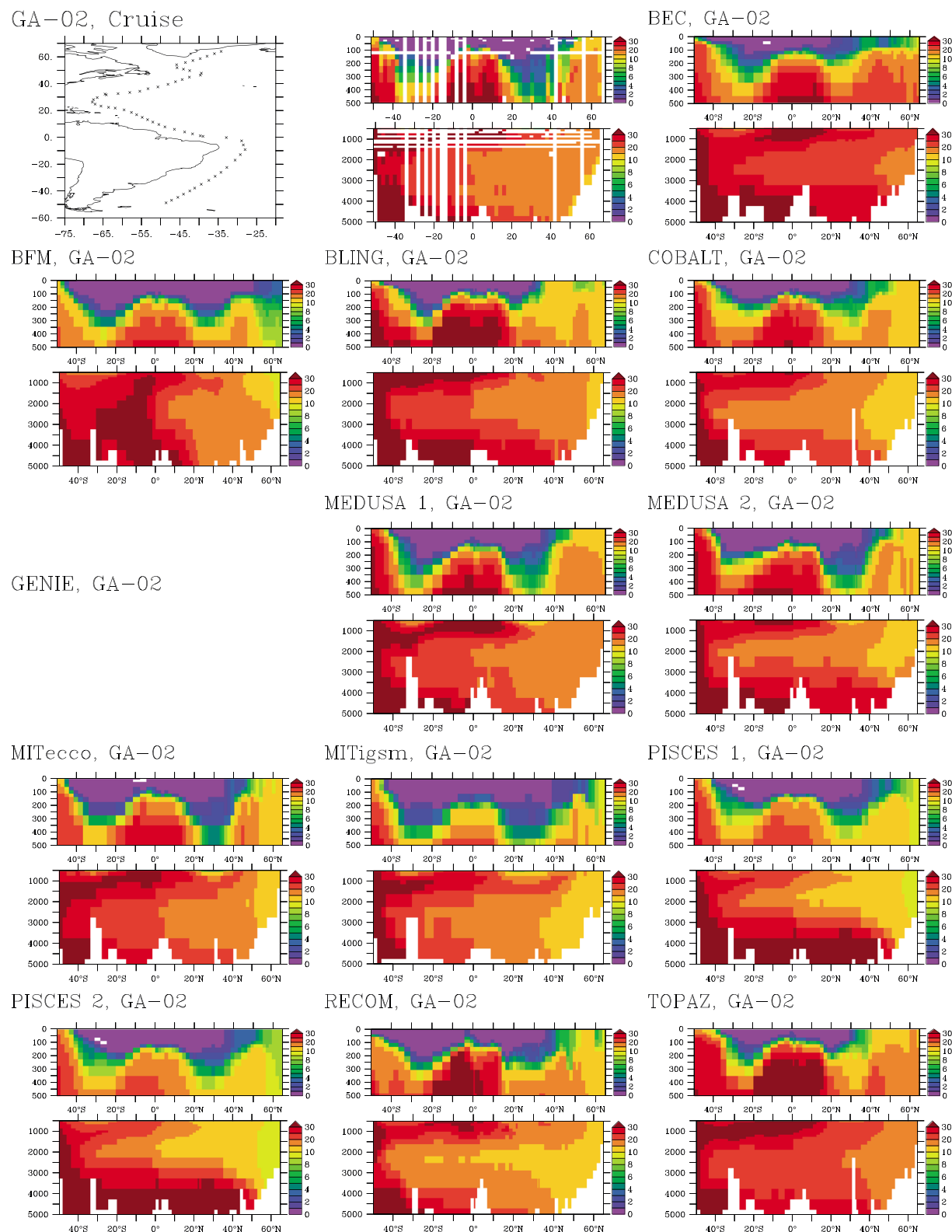
Figure 9. \text{NO}_3 concentrations ( \mu\text{M} ) from the GA-02 cruise [Rijkenberg et al., 2014] and extracted from the FeMIP models ( \text{NO}_3 data not provided for GENIE).
