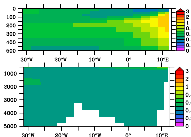
MITigsm, CoFeMUG
