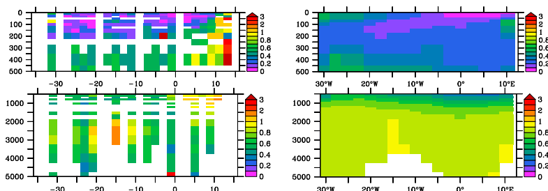
BLING, CoFeMUG
