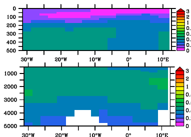
MEDUSA 1, CoFeMUG
