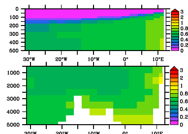
PISCES 2, CoFeMUG
