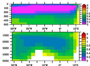
MEDUSA 2, CoFeMUG
