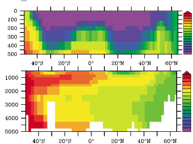
RECOM, GA-02
