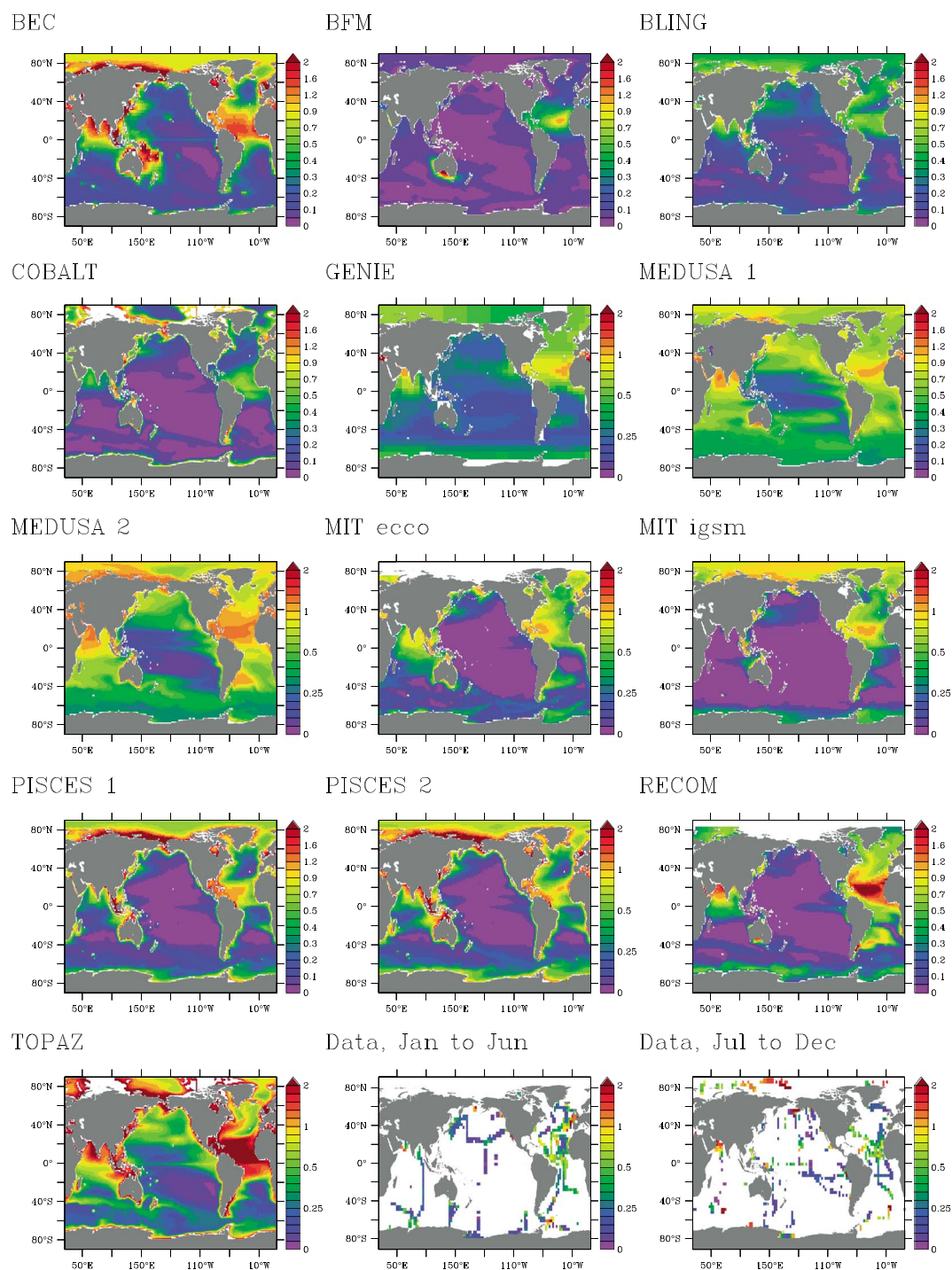
Figure 2. Annual mean DFe concentrations (nM) averaged over the upper 50 m from the FeMIP models. Data averaged over the period January to June and July to December are taken from the expanded Tagliabue et al. [2012] data set and have been averaged over 5° bins in latitude and longitude to improve visibility.
