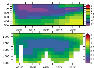
MEDUSA 2, GA-03
