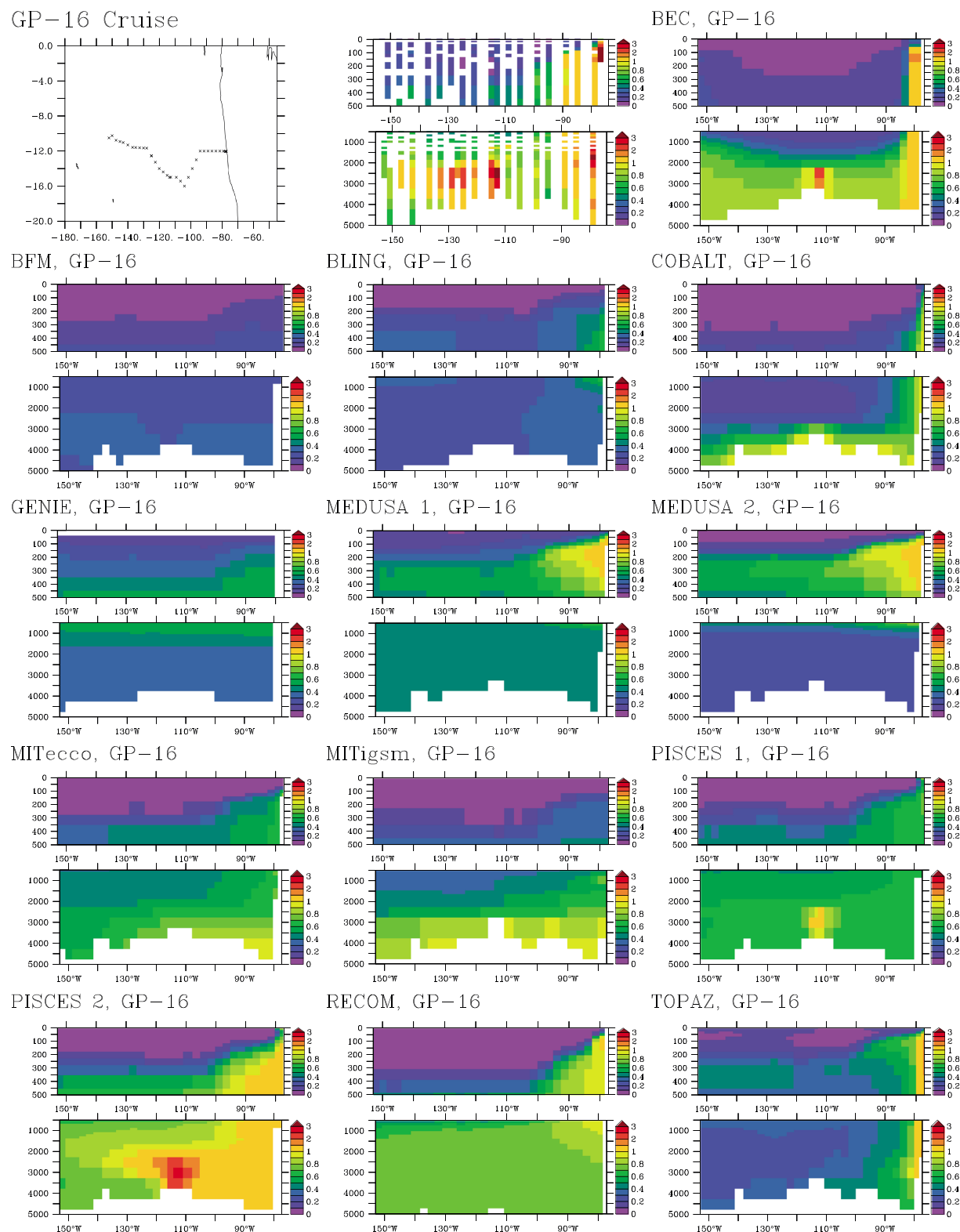
Figure 7. DFe concentrations (nM) from the GP-16 cruise [Resing et al., 2015] and extracted from the FeMIP models.
