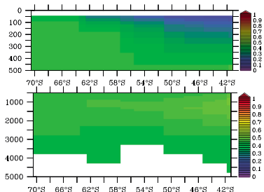
MITeco, GIPY-5
