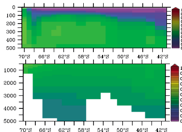
MEDUSA 1, GIPY-5
