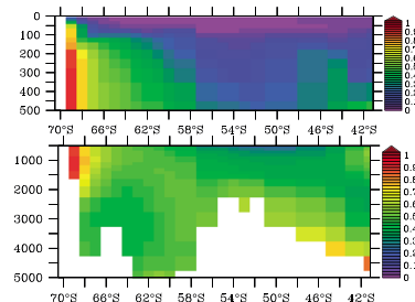
MEDUSA 2, GIPY-5
