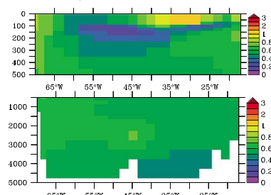
TOPAZ, GA-03
