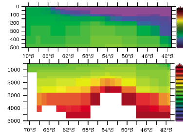
RECOM, GIPY-5
