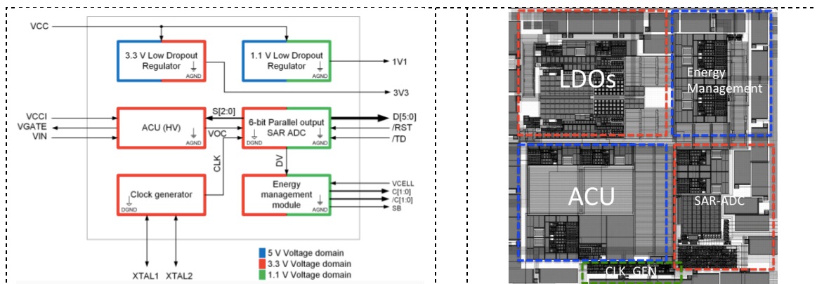
Figure 2. ASIC1 envisaged version and implementation.
