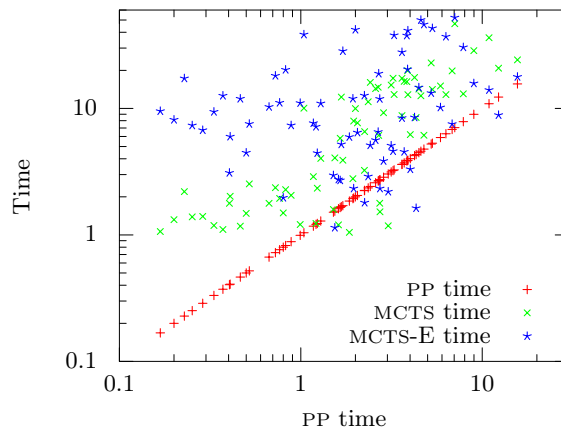
Fig. 1. Time needed to solve various opening positions in the game of \gamma .
