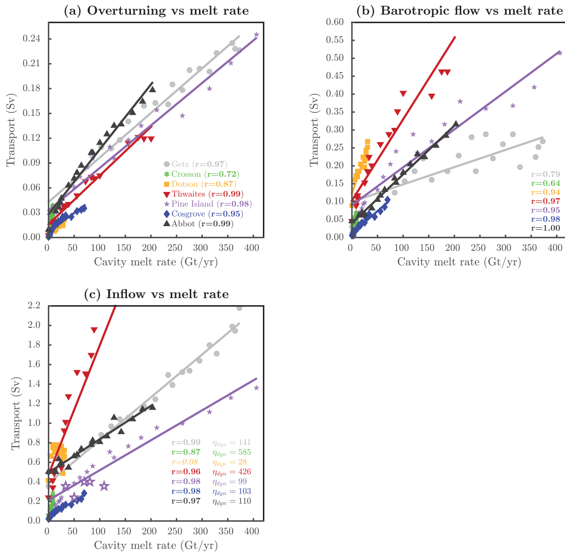
Figure 7. (a) Amplitude of the overturning circulation versus melt in each cavity across the 18 simulations with varying ( C_d\Gamma_T ) values. The overturning circulation is estimated through the sections indicated in white in Figure 1, and calculated as the along-z maximum of |\int_{z_b}^z \int u \cdot dx \cdot dz| where z_b is the bottom depth, u the ocean velocity perpendicular to the section, and x the direction along the section. (b) Same as Figure 7a but for the amplitude of the barotropic transport within each cavity, which is calculated as the maximum amplitude (maximum minus minimum) of the barotropic stream function (BSF) under the ice-shelf. (c) Positive seawater transport through the ice-shelf front (positive into the cavity) calculated from daily velocities then averaged over year 5. The lines are least-mean-square regressions, and corresponding correlations ( r ) are indicated on the lower-right corner (all of them with statistical significance greater than 99%). In Figure 7c, \eta_{dyn} represents the dynamical efficiency, i.e., the slope expressed in Sv/Sv (see Appendix C for more details on \eta_{dyn} ), and the empty stars correspond to the observational estimates by Dutrieux et al. [2014].
