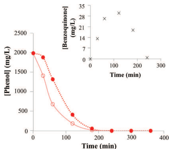
Fig. 5. Comparison of the variation of the phenol concentration during electrolysis in the presence (full symbol) and in the absence of activated carbon (empty symbol). C^0 = 1985 mg/L, m_{A.C.} = 2 g, anode: BDD, i = 0.215 A/cm 2 , V = 100 mL, T = 30 °C, pH = 13 . Inset panel: variation of p -benzoquinone concentration during electrolysis.
