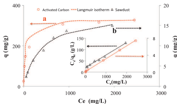
Fig. 2. Experimental data and modeling of the equilibrium adsorption isotherms of phenol on activated carbon (a) and sawdust (b) at 30 °C. (a) m A.C. = 5 g, V = 250 mL, C° = 500–9000 mg/L; (b) m sawdust = 1 g, V = 100 mL, C° = 100–2115 mg/L. Inset panel: Linearization of Langmuir equations for the adsorption of phenol on adsorbents at 30 °C.
