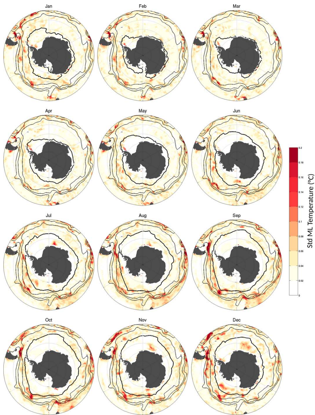
Figure A4. Standard deviation of the mixed-layer temperature from the 100 Monte Carlo experiments (in °C).
