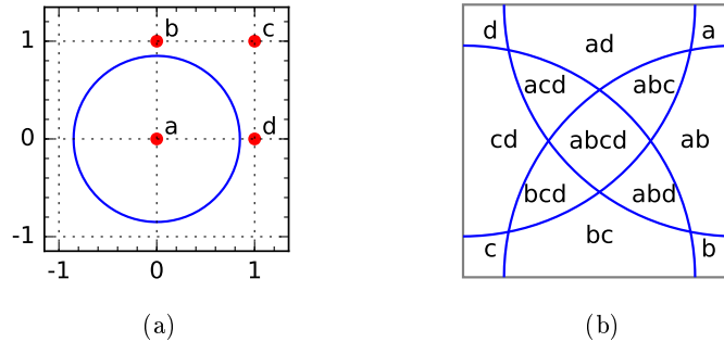
Fig. 2: (a) A circle with diameter 1.7 and the four pixels in the toggling boundary (which is equal to the grid boundary): a , b , c , d . (b) The (flatten) dual of the closed disc bounded by the circle. Among the 16 = 2^4 potential digitizations provided by the 4-pixels a , b , c , d , three of them does not actually appear ( \emptyset , ac and bd ) and some others appear multiple times (the four singular digitizations, which are obviously congruent, and the vertical and horizontal pairs which each appear twice). Eventually, there are only 8 digitizations (and actually the (sewed) dual is divided into 8 regions).
