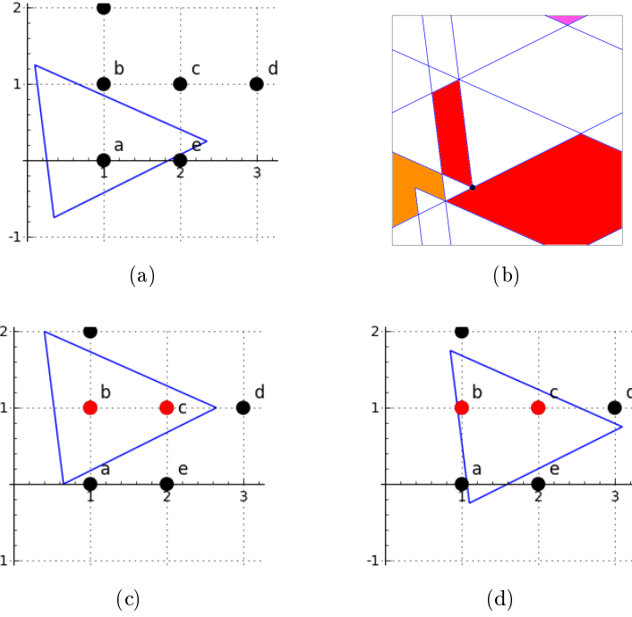
Fig. 4: (a) A triangle and its toggling boundary. (b) The dual of the (filled) triangle. The four colored regions correspond to the same digitization: the horizontal pair. Moreover, the two red regions belong to the same cell of the partition \bigwedge_{p \in \mathfrak{B}} \Gamma_p , the cell associated to the digitization bc (these two regions are separated by the unique point of the cell abcd ). The orange region is the cell cd and the pink region is the cell ae . (c), (d) The configurations of the shifted triangle in the two red regions. Since they are disconnected, it is not possible to continuously move to one configuration to the other without hurting a black toggling point. Note that the triangle could be slightly inflated so as to provide a strictly convex counterexample.
