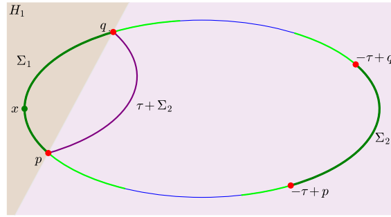
Fig. 5: Light green: the arcs \Gamma_1 and \Gamma_2 .
