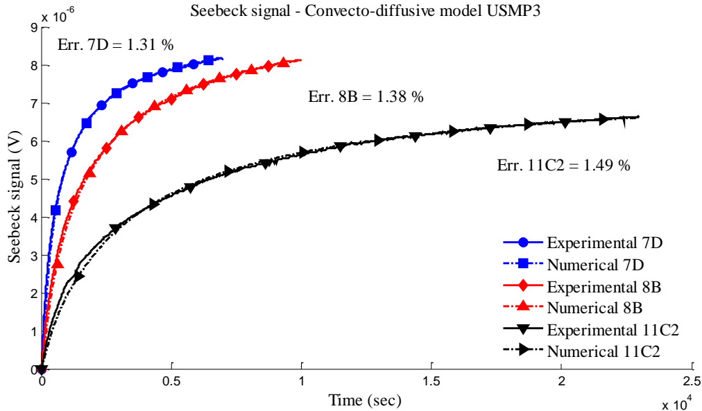
Figure 5: Time evolution of the Seebeck signal recorded in the Mephisto USMP3 experiments during the re-homogenization period, compared to the results obtained by simulation using the convecto-diffusive model (adjustment of the coefficient \alpha and of the Seebeck coefficient).
