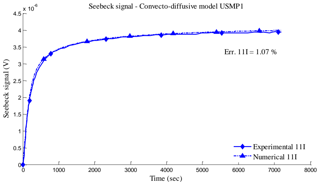
Figure 6: Time evolution of the Seebeck signal in the Mephisto USMP1 11I experiment during the re-homogenization period, compared to the result obtained by simulation using the convecto-diffusive model (adjustment of the Seebeck coefficient; the coefficient \alpha is determined from the USMP3 simulations).
