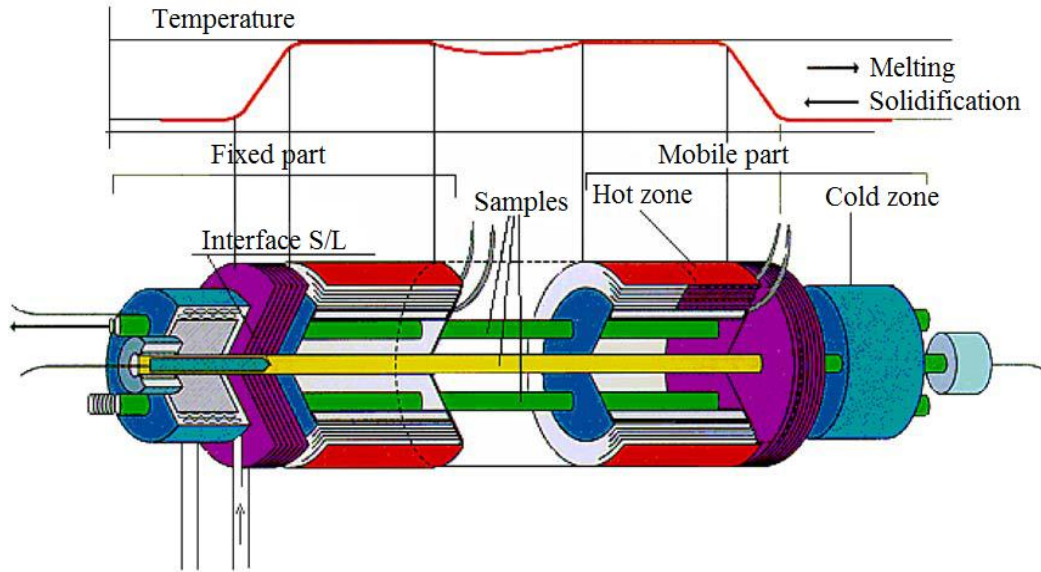
Figure 1: Schematic of the Mephisto furnace, showing the implementation of the three samples within the fixed and mobile parts. The solid-liquid interface is located between the hot and cold zones. The characteristic temperature profile, as given by the position of the hot and cold zones is also indicated, along with the directions of melting and solidification.
