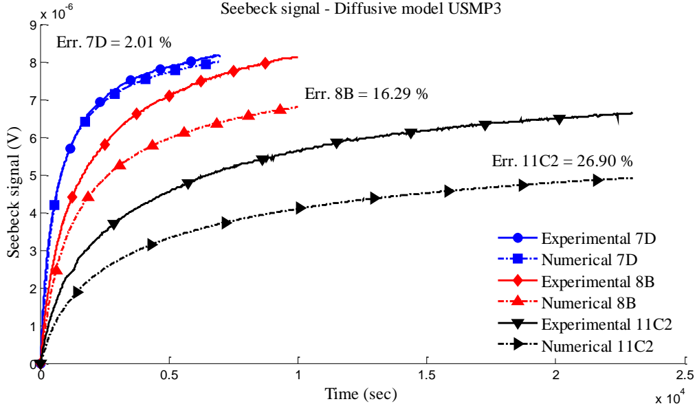
Figure 4: Time evolution of the Seebeck signal recorded in the Mephisto USMP3 experiments during the re-homogenization period, compared to the results obtained by simulation using the purely diffusive transient model ( \alpha = 0 ).
