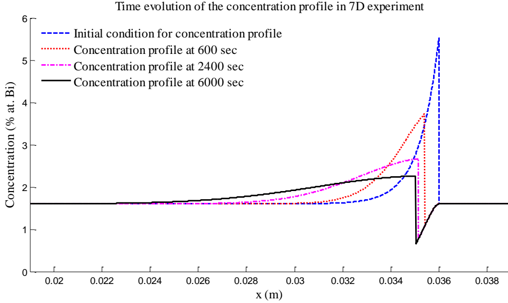
Figure 3: Time evolution of the longitudinal concentration profile in the 7D experiment obtained by simulation using the purely diffusive transient model ( \alpha = 0 ). The concentration profile used as an initial condition for the simulation (i.e. at 0 sec) is plotted with blue dashed line, and the concentration profiles corresponding to 600 sec, 2400 sec and 6000 sec are plotted with red dotted line, magenta dashed-dotted line and black solid line, respectively. The solidification occurs from right to left.
