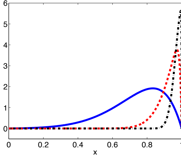
Figure 12: The optimal initial condition y_0 in (0, L) for \varepsilon = 10^{-1} (full line), \varepsilon = 10^{-2} (dashed line) and \varepsilon = 10^{-3} (dashed-dotted line) and T = -M = L = 1 ; r = h^2 - h = 1/320 .
