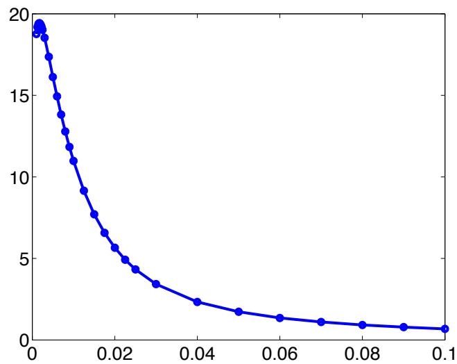
Figure 8: Cost of control K(\varepsilon, T, M) w.r.t. \varepsilon \in [10^{-3}, 10^{-1}] for T = L/M and L = M = 1 ; r = h^2 - h = 1/320 .
