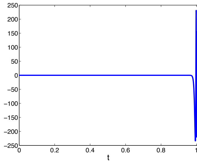
Figure 6: Approximation \lambda_h(0, t) of the control w.r.t. t \in [0, T] for \varepsilon = 10^{-3} and T = L = -M = 1 ; r = h^2 - h = 1/320 .
