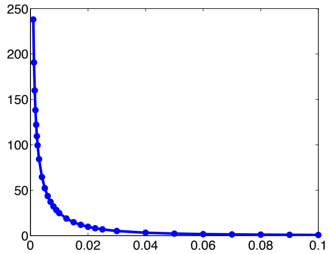
Figure 7: Cost of control K(\varepsilon, T, M) w.r.t. \varepsilon \in [10^{-3}, 10^{-1}] for T = 0.95L/M and L = M = 1 ; r = h^2 - h = 1/320 .
