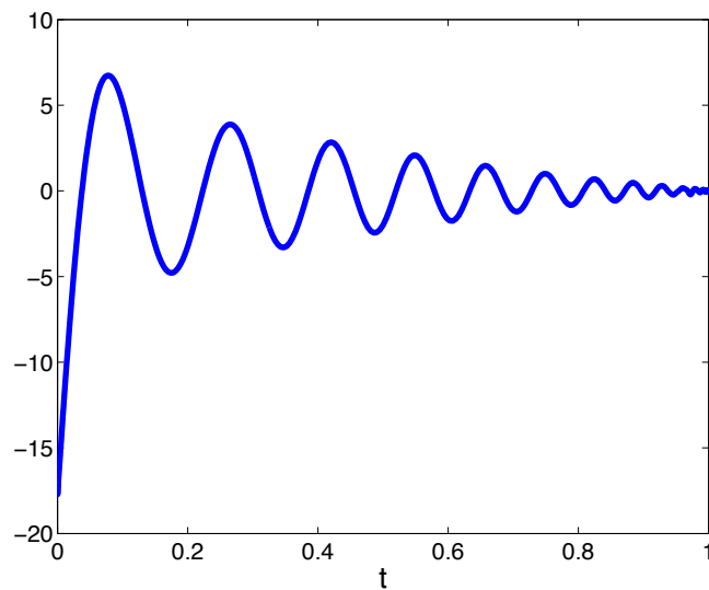
Figure 2: Approximation \lambda_h(0, t) of the control w.r.t. t \in [0, T] for \varepsilon = 10^{-2} and T = L = M = 1 ; r = h^2 - h = 1/320 .
