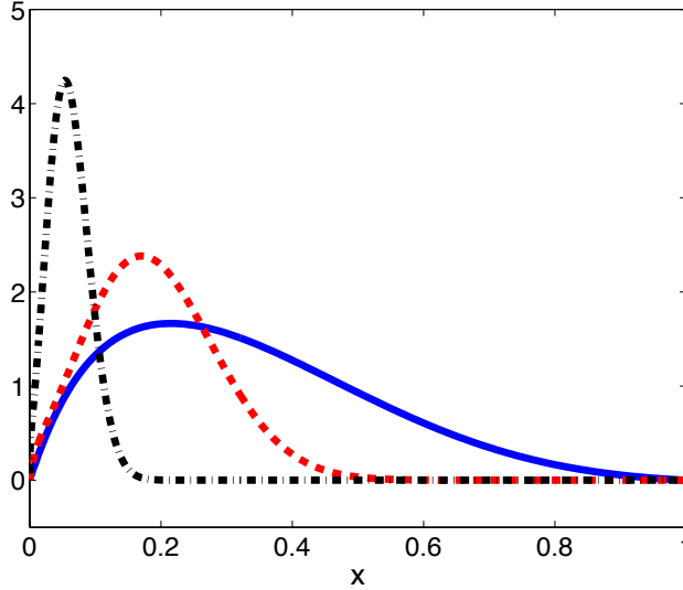
Figure 11: The optimal initial condition y_0 in (0, L) for \varepsilon = 10^{-1} (full line), \varepsilon = 10^{-2} (dashed line) and \varepsilon = 10^{-3} (dashed-dotted line) and T = M = L = 1 ; r = h^2 - h = 1/320 .
