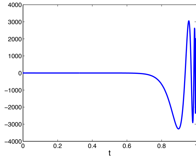
Figure 5: Approximation \lambda_h(0, t) of the control w.r.t. t \in [0, T] for \varepsilon = 10^{-2} and T = L = -M = 1 ; r = h^2 - h = 1/320 .
