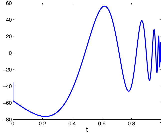
Figure 4: Approximation \lambda_h(0, t) of the control w.r.t. t \in [0, T] for \varepsilon = 10^{-1} and T = L = -M = 1 ; r = h^2 - h = 1/320 .
