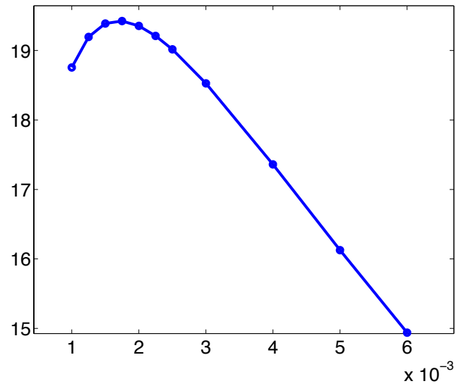
Figure 9: Cost of control K(\varepsilon, T, M) w.r.t. \varepsilon \in [10^{-3}, 6 \times 10^{-3}] for T = 0.95L/M and L = M = 1 ; r = h^2 - h = 1/320 .
