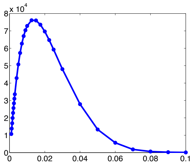
Figure 14: Cost of control K(\varepsilon, T, M) w.r.t. \varepsilon \in [10^{-3}, 10^{-1}] for T = L/M and L = -M = 1 ; r = h^2 - h = 1/320 .
