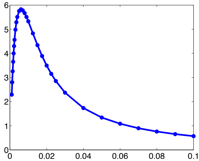
Figure 10: Cost of control K(\varepsilon, T, M) w.r.t. \varepsilon \in [10^{-3}, 10^{-1}] for T = 1.05L/M and L = M = 1 ; r = h^2 - h = 1/320 .
