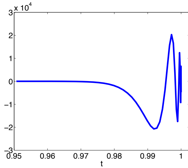
Figure 13: Approximation \lambda_h(0, t) of the corresponding control w.r.t. t \in [0, T] for \varepsilon = 10^{-3} and T = L = -M = 1 ; r = h^2 - h = 1/320 .
