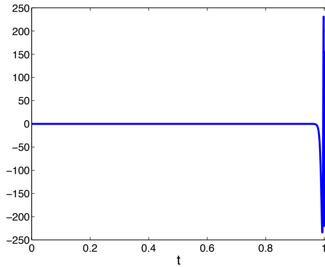
Figure 6: r = h^2 - h = 1/320 - T = 1 L = 1 = -M ; Control for \varepsilon = 10^{-3} .
