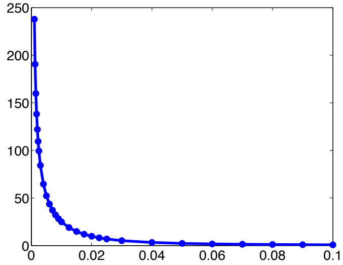
Figure 7: r = h^2 - h = 1/320 - T = 0.95 L = 1 = M ; K(\varepsilon, T, M) vs. \varepsilon \in [10^{-3}, 10^{-1}] .
