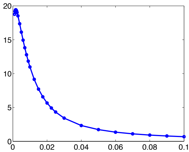
Figure 8: r = h^2 - h = 1/320 - T = 1 . L = 1 = M ; K(\varepsilon, T, M) vs. \varepsilon \in [10^{-3}, 10^{-1}] .
