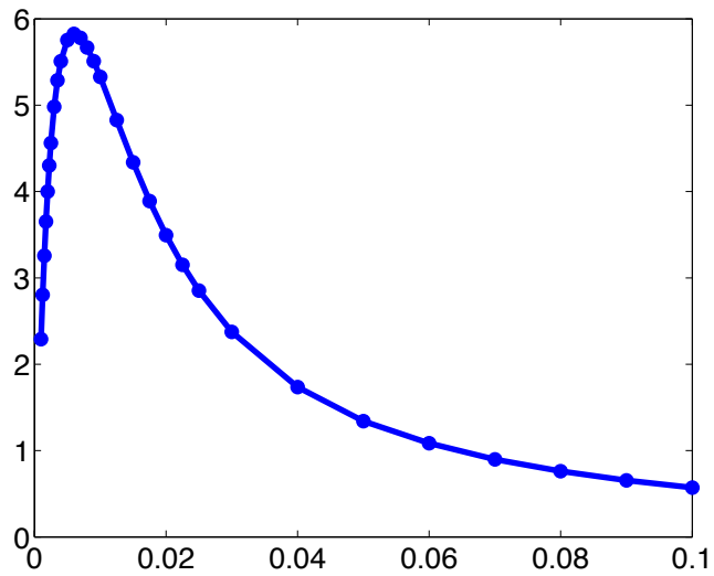
Figure 10: r = h^2 - h = 1/320 - T = 1.05 - M = 1 ; K(\varepsilon, T, M) vs. \varepsilon \in [10^{-3}, 10^{-1}] .
