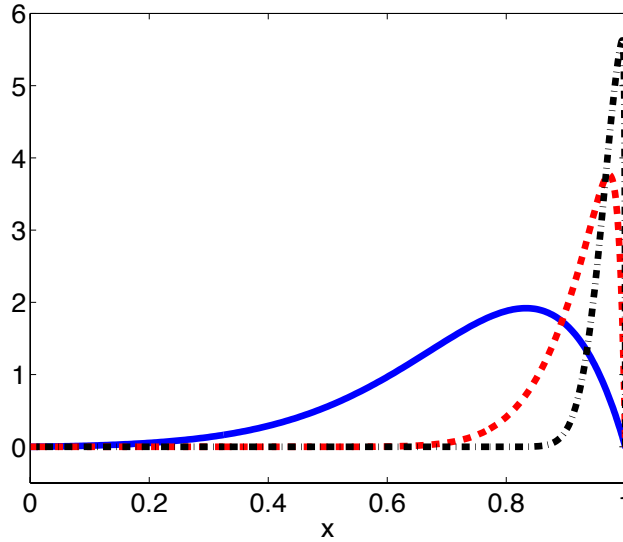
Figure 12: r = h^2 - h = 1/320 - T = 1 - M = -1 - The optimal initial condition y_0 in \Omega for \varepsilon = 10^{-1} (full line), \varepsilon = 10^{-2} (dashed line) and \varepsilon = 10^{-3} (dashed-dotted line).
