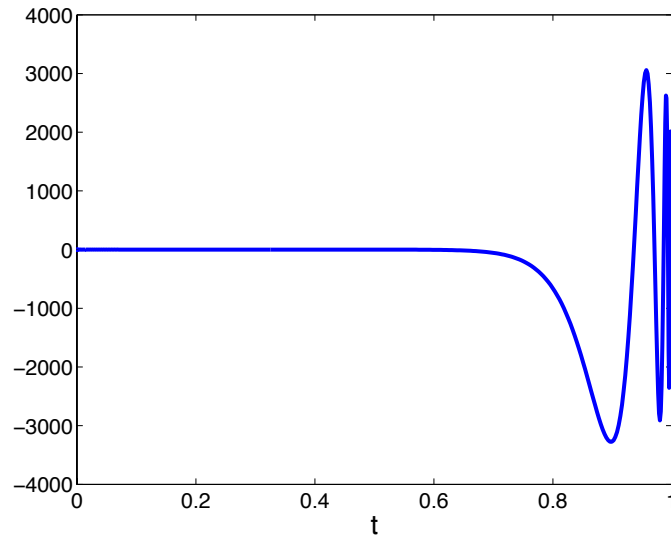
Figure 5: r = h^2 - h = 1/320 - T = 1 L = 1 = -M ; Control for \varepsilon = 10^{-2} .
