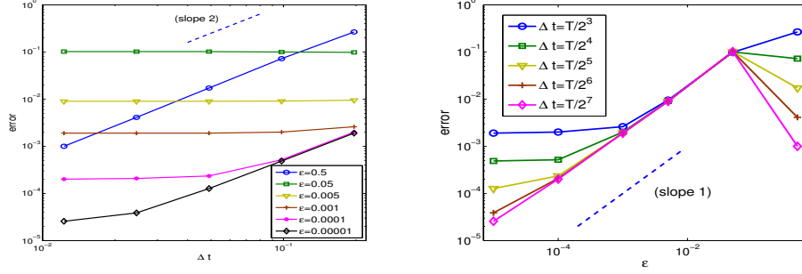
Figure 1: Temporal error of SIRC-PIC at T = \pi/2 with respect to \Delta t = H = O(h) and \varepsilon : maximum error in the density \rho^\varepsilon .
