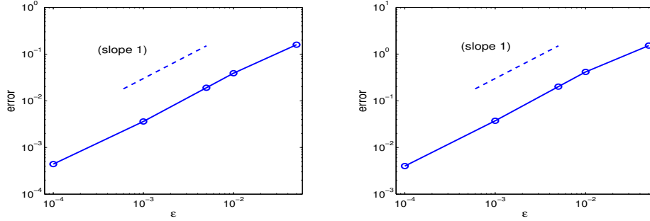
Figure 2: Convergence from the Vlasov-Poisson equation (1.1) to the limit model (1.3): maximum error with respect to \varepsilon at T = \pi/2 in the density \rho^\varepsilon (left) and in the kinetic energy density \rho_v^\varepsilon (right).
