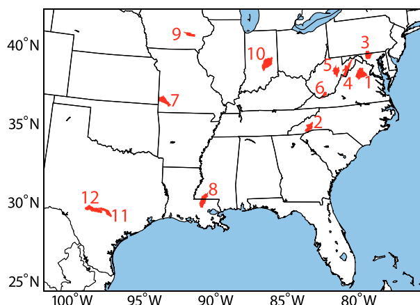
Figure 1. Locations of the 12 MOPEX catchments in the Eastern United States.
