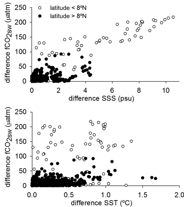
Figure 4. Comparison of the difference in fCO_{2sw} , salinity (SSS), and temperature (SST) among consecutive voyages of the MN Colibri with a time lag lower than a week between cruises. Values were averaged every 1/20 latitudinal degrees prior comparison. Data at latitudes lower than 8°N are represented with white dots, and black dots represent data at latitudes higher than 8°N.
