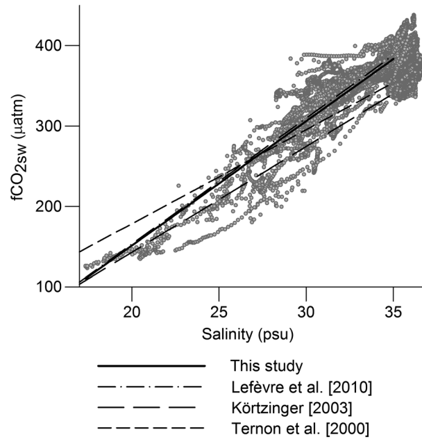
Figure 3. fCO_{2sw} as a function of SSS for the 30 voyages of the MN Colibri . Linear regression of fCO_{2sw} and SSS for salinities lower than 35 psu is shown (solid line) along with the relationships of Ternon et al. [2000], Körtzinger [2003], and Lefèvre et al. [2010] for the Amazon plume.
