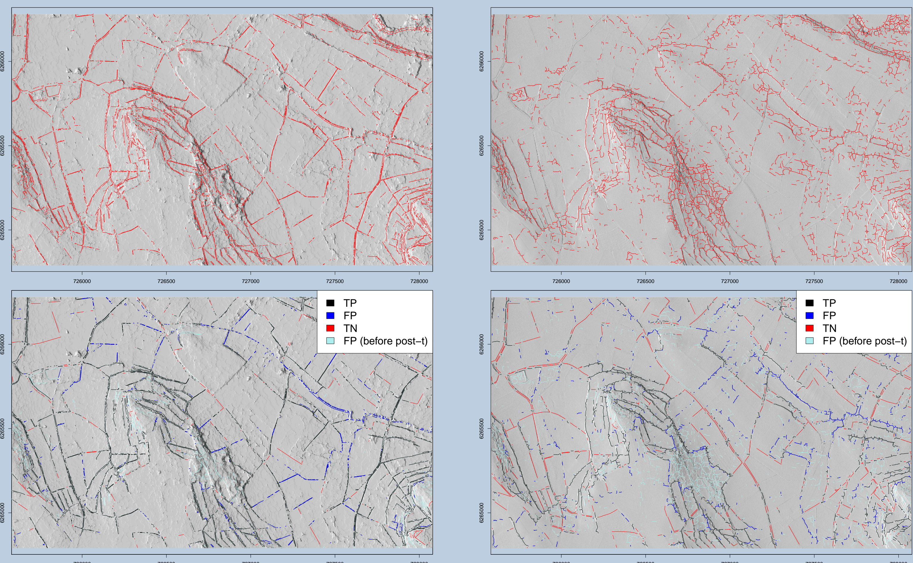
Figure 3: Maps of the detected terrace slope of LiDAR DTM using the LSD method (left) and from the Pleiades DSM when using the geomorphometric method (right). Resulting TP elements in black, TN elements in red, filtered FP elements in blue and non filtered FP elements in light blue (down)
