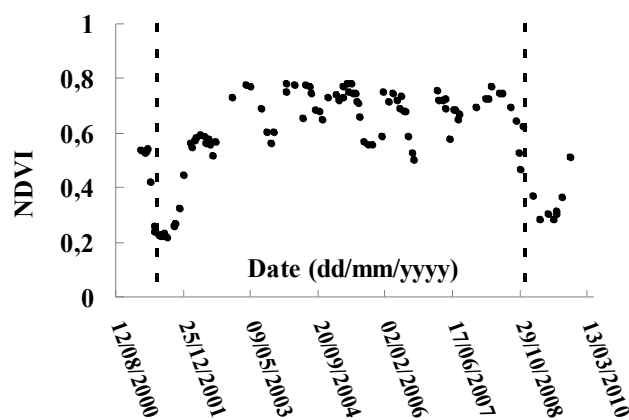
Figure 3: Landsat NDVI time-series of a given Eucalyptus stand. Dashed line indicates the planting date.
