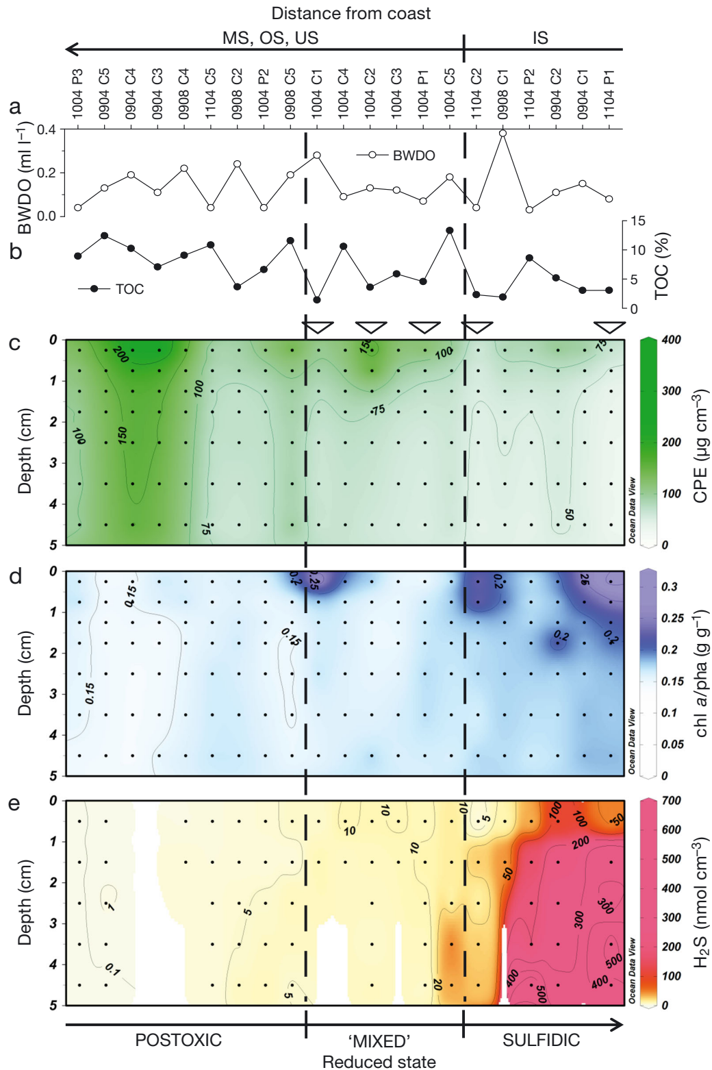
Fig. 4. Geochemical conditions along a fixed redox gradient. (a) Bottom-water dissolved oxygen (BWDO), (b) surface total organic carbon (TOC), and vertical profiles (0 to 5 cm) of (c) chloroplastic pigment equivalents (CPE), (d) ratio of chlorophyll a to phaeopigments (chl a/pha) and (e) pore water sulfide ( \text{H}_2\text{S} ) along the increasing \Sigma\text{H}_2\text{S}_{[2]} gradient. Top horizontal axis in (a) indicates the year, month and station sample. Vertical bars: redox states; triangles: sample sites with Thioploca spp. mats. IS: inner shelf; MS: middle shelf; OS: outer shelf; US: upper slope
