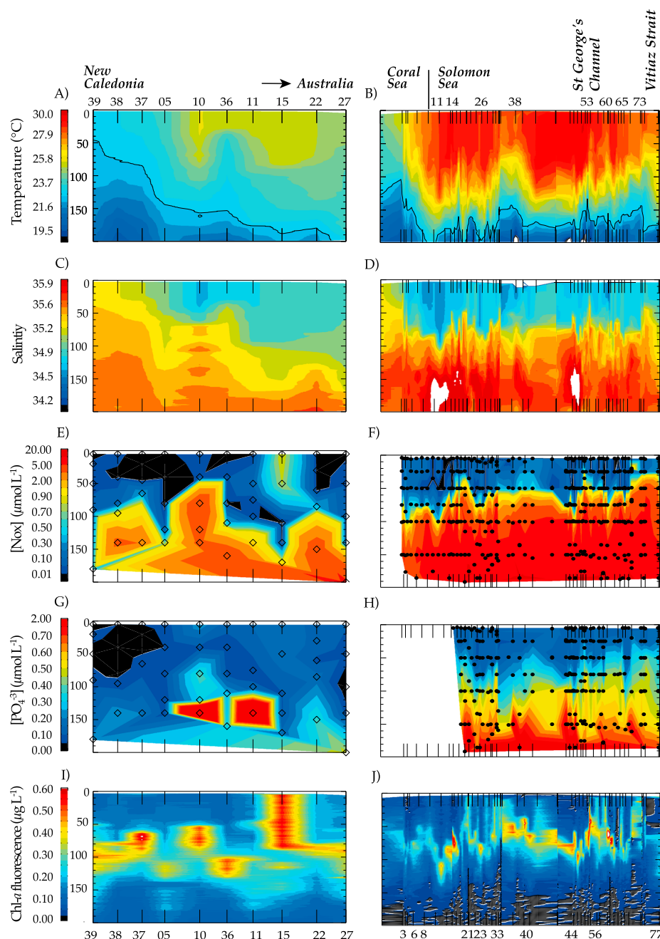
Figure 3. Horizontal and vertical distributions of physicochemical parameters during the (left) Bifurcation cruise and the (right) Pandora cruise: (a and b) temperature ( ^{\circ}\text{C} ), (c and d) salinity, (e and f) \text{NO}_x concentrations ( \mu\text{mol L}^{-1} ), (g and h) \text{PO}_4^{3-} concentrations ( \mu\text{mol L}^{-1} ), and (i and j) Chlorophyll a fluorescence ( \mu\text{g L}^{-1} ). Station numbers are reported on the top and bottom of panels.
