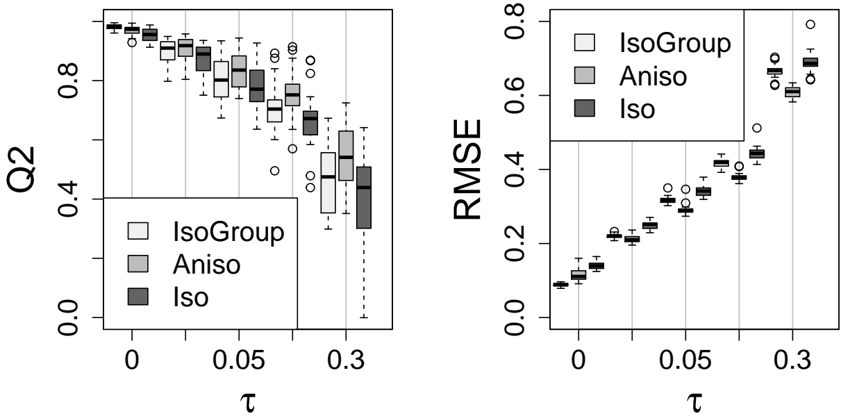
Figure 5: Prediction quality of the model with an isotropic by group kernel found by Algorithm 4 (IsoGroup) anisotropic kernel (Aniso) and isotropic kernel (Iso) according to the value of a nugget effect added in the simulated model. 25 trajectories are simulated for a learning set of size \{160\} . The prediction quality criteria are Q2 and RMSE.
