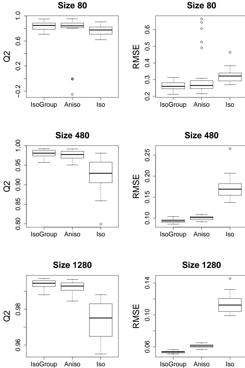
Figure 3: Prediction quality of the model with an isotropic by group kernel found by Algorithm 4 on the left, anisotropic kernel in the middle and isotropic kernel on the right according to the sample size. 25 trajectories are simulated for each learning set size \{80, 480, 1280\} . The criteria of prediction quality are Q2 and RMSE.
