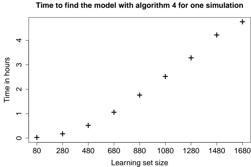
Figure 1: Time in hours to find the best model with the Algorithm 4 . 25 trajectories are simulated for the each size \{80, 280, 480, 680, 880, 1080, 1280, 1480, 1680\} .
