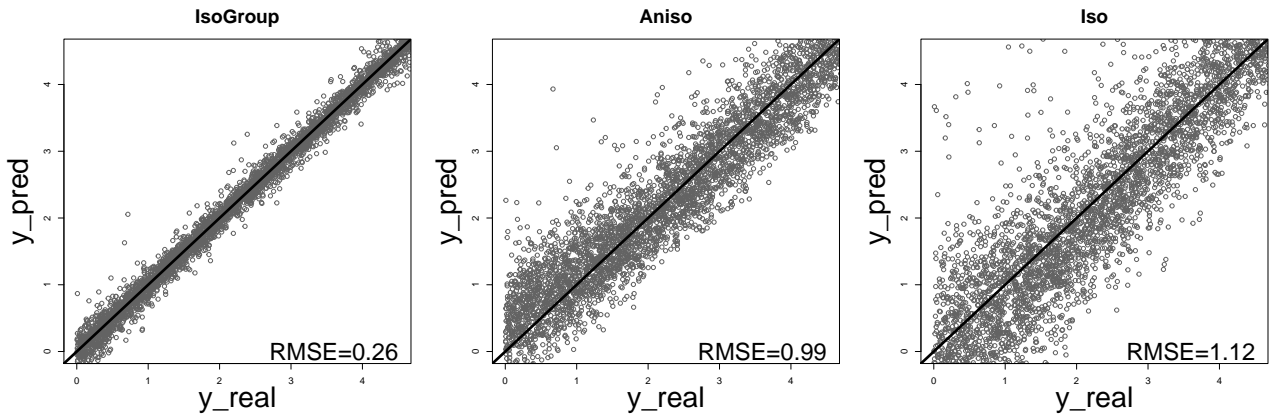
Figure 6: Kriging prediction plots for the function : isotropic by group kernel (left), anisotropic kernel (middle), isotropic kernel (right).
