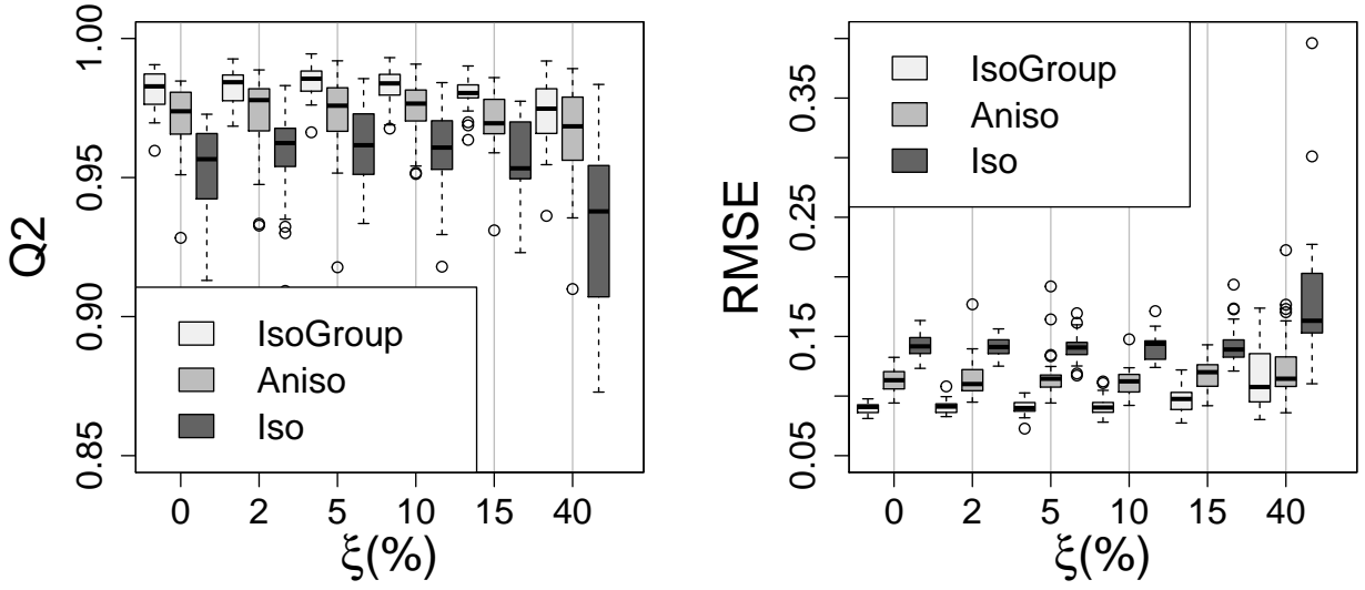
Figure 4: Prediction quality of the model with an isotropic by group kernel found by Algorithm 4 (IsoGroup) anisotropic kernel (Aniso) and isotropic kernel (Iso) according to an error added on the range parameters in the simulated model. 25 trajectories are simulated for a learning set of size 400. The prediction quality criteria are Q2 and RMSE.
