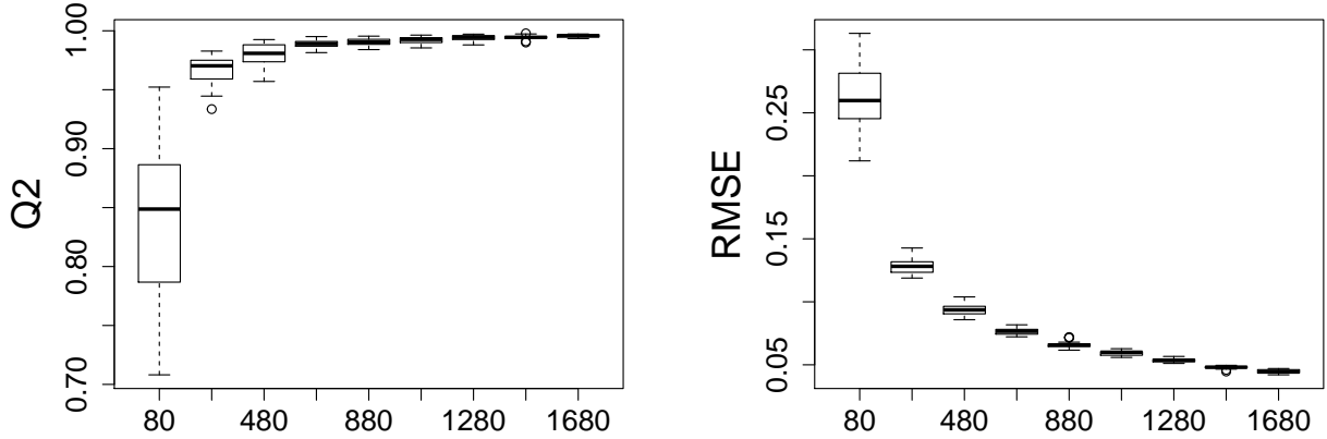
Figure 2: Prediction quality of the model with an isotropic by group kernel found by Algorithm 4 according to the sample size. 25 trajectories are simulated for each size \{80, 280, 480, 680, 880, 1080, 1280, 1480, 1680\} . The criteria of prediction quality are Q2 and RMSE.
