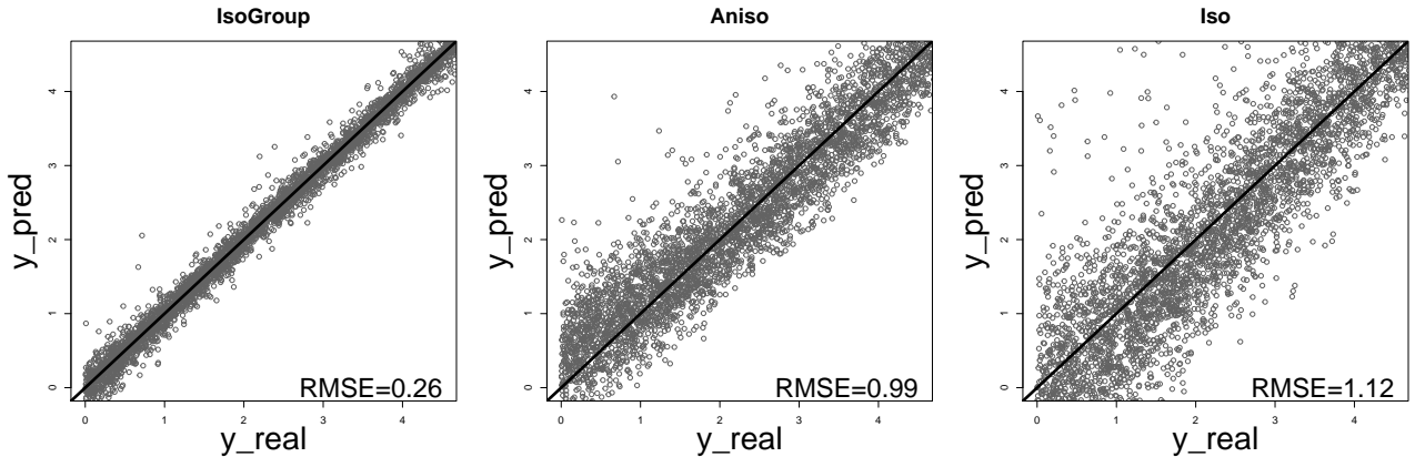
Figure 6: Kriging prediction plots for the function : isotropic by group kernel (left), anisotropic kernel (middle), isotropic kernel (right).
