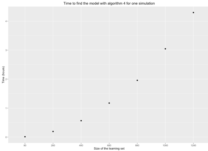
Figure 1: Time in hours to find the best model with the Algorithm 4 . 25 trajectories are simulated for the each size \{80, 280, 480, 680, 880, 1080, 1280\} .
