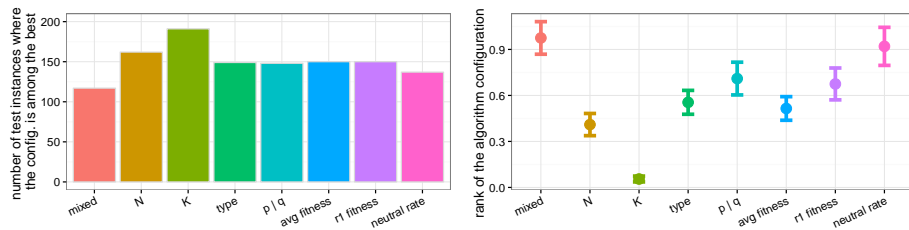
Fig. 5. Number of test instances (out of 200) where the baseline configuration (mixing all training instances) and each feature-based configuration (partitioning training instances) is not statistically outperformed by any other (left), and rank of each configuration over all test instances (right).
