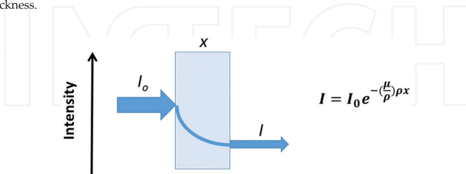
Figure 2. Sketch for the X-Ray absorption measurement in transmission mode.
