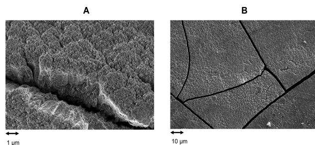
Figure 2. SEM images of a pristine nanoparticulate \text{SnO}_2 electrode (A) and an initially cycled electrode in LiTFSI (B). The columnar electrode structure (A) and the crack forming caused by the volume expansion during cycling (B) are illustrated.
