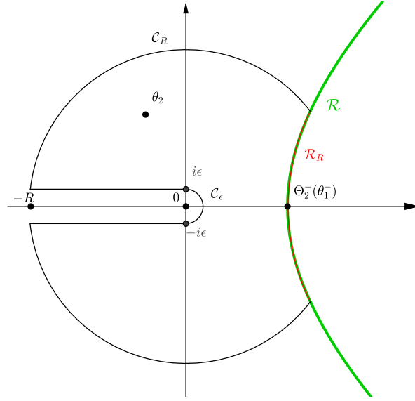
Figure 12: Integration contour used in the proof of Theorem 23
