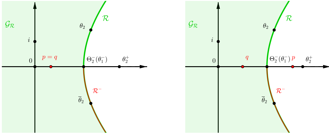
Figure 7: The curve \mathcal{R} in (20) is symmetric w.r.t. the horizontal axis, and \mathcal{G}_R is the domain in green. The curve \mathcal{R}^- is the half branch of \mathcal{R} with negative imaginary part. The points p and q are used to define the conformal mapping W , see (18) and (27). The point q is defined as follows: if the pole p is in \mathcal{G}_R then q = p (figure on the left), otherwise q = \frac{1}{2}\Theta_2^-(\theta_1^-) (figure on the right), see (25)
