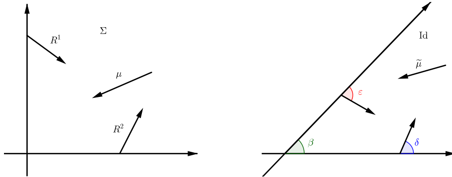
Figure 13: The linear transformation T in (54) from the quadrant to the wedge of opening angle \beta
