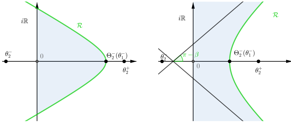
Figure 6: On the left \sigma_{12} < 0 , and on the right \sigma_{12} \geq 0 . The blue domain is the set \overline{\mathcal{G}_R} \cap \{\theta_2 \in \mathbb{C} : \Re \theta_2 > 0\} . On the right, the two lines are the asymptotes to \mathcal{R}
