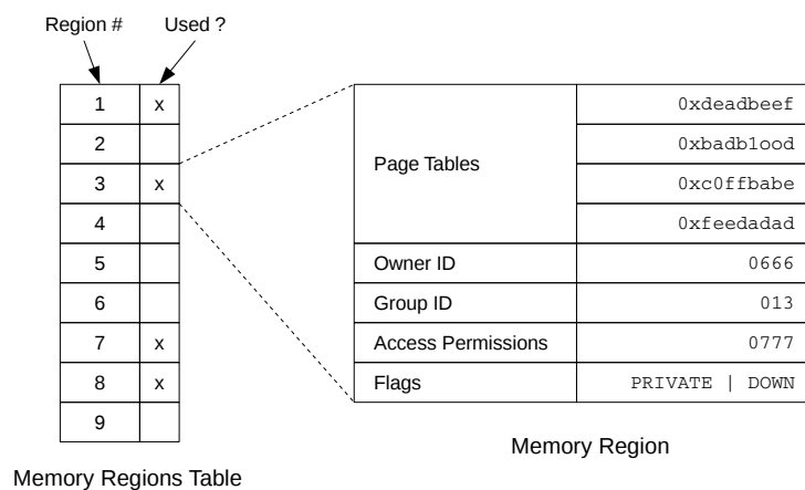
Figure 7: Memory region.
