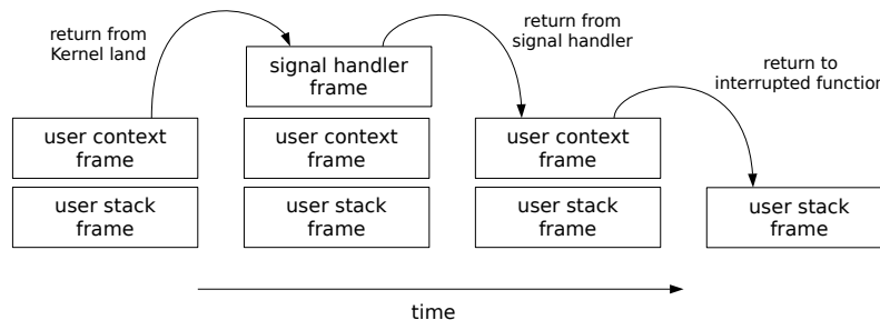
Figure 5: Signal stack.
