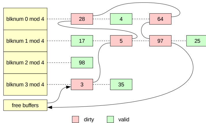
Figure 10: Buffer cache.
