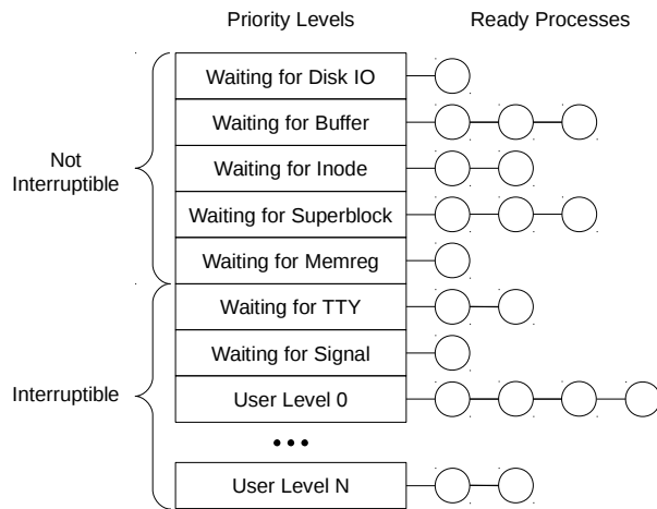
Figure 4: Scheduler queues.
