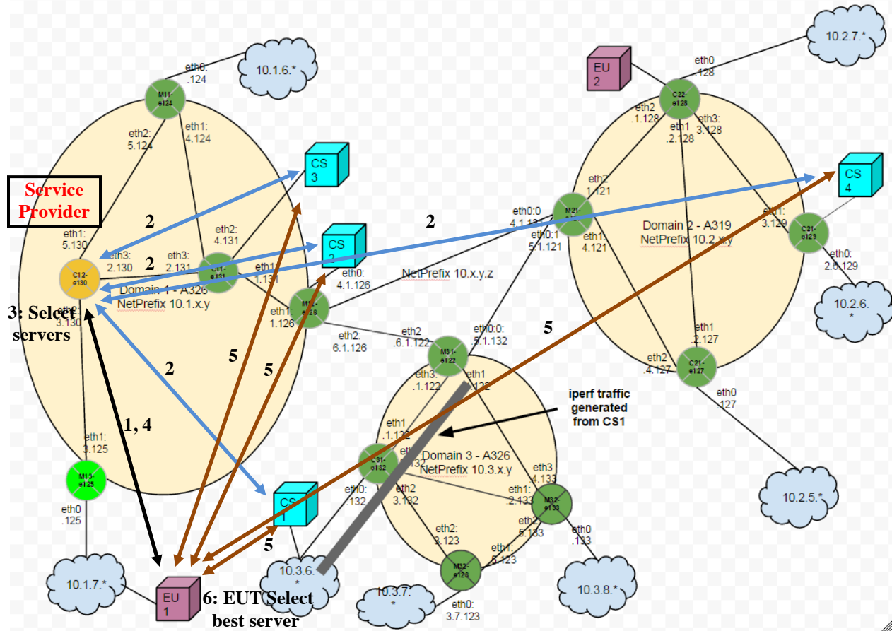
Figure 2. DISEDAN System testbed; interactions between system's modules
