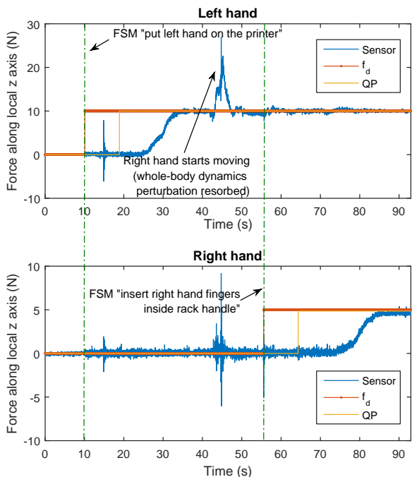
Fig. 11. Printer tray opening with HRP-4.
