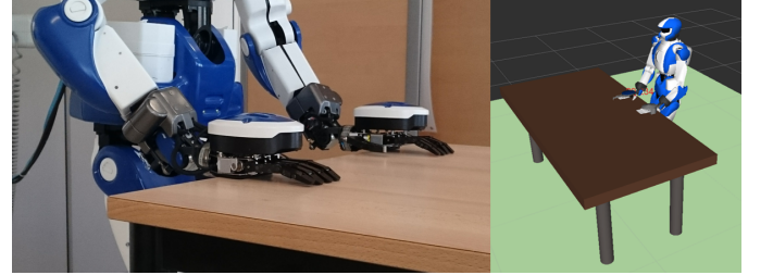
Fig. 6. Base experiment for comparing the different proposed QP force control paradigms. Each hand is controlled with a different paradigm.
