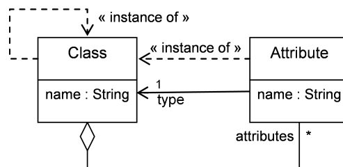
Figure 4: M2 layer – Class and Attribute classes.
