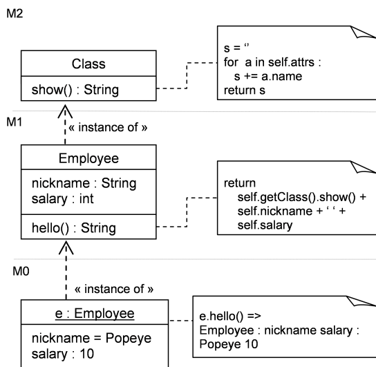
Figure 1: Employee class, version 1
