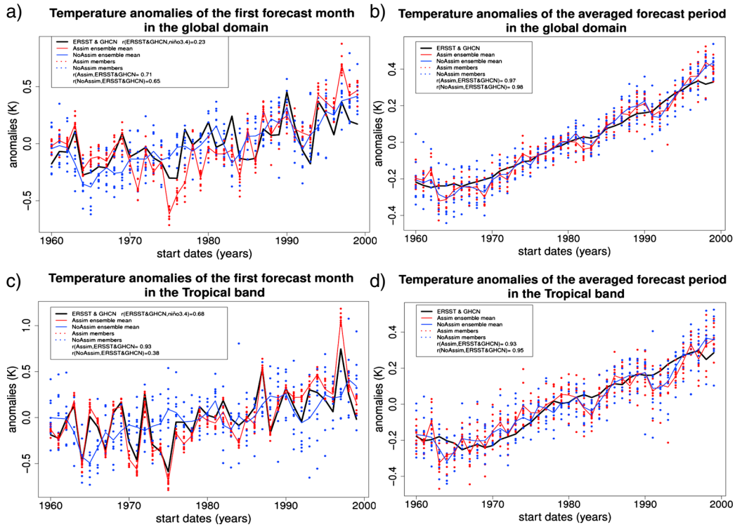
Figure 2. Anomaly time series of Assim and NoAssim near-surface temperature with GHCN and ERSST in the (a,b) global domain and (c,d) tropical band. Figure 2a shows the time series of the first forecast month with a spatial average over the whole global domain; Figure 2b is the anomalies time series of the 120 forecast months average over the whole global domain. In solid black are the reference data. Assim ensemble mean anomalies are in solid red, while the Assim ensemble members in dotted red. Analogously, the NoAssim ensemble mean anomalies are in solid blue, and the NoAssim ensemble members in dotted blue. Figures 2c and 2d are the same as Figures 2a and 2b, but in tropical band. The year in the abscissa corresponds to the start date of each individual hindcast. Note that the legend indicates the correlation of Assim with the reference data and the correlation of NoAssim with the reference data. In Figures 2a and 2c, the correlation between the observed Niño 3.4 SST index with the tropically averaged reference data is also shown.
