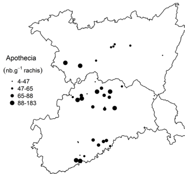
Figure 3. Density of H. fraxineus apothecia in the soil litter (number per g of ash rachis dry weight, i.e. ADW).
