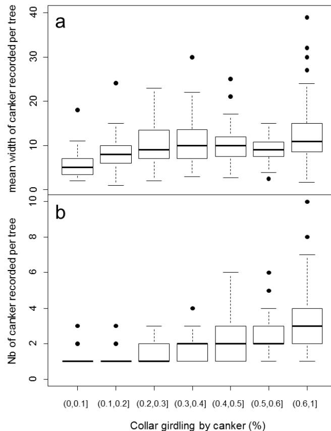
Figure 4. Number and width of lesions observed on the collar of individual ash trees.
