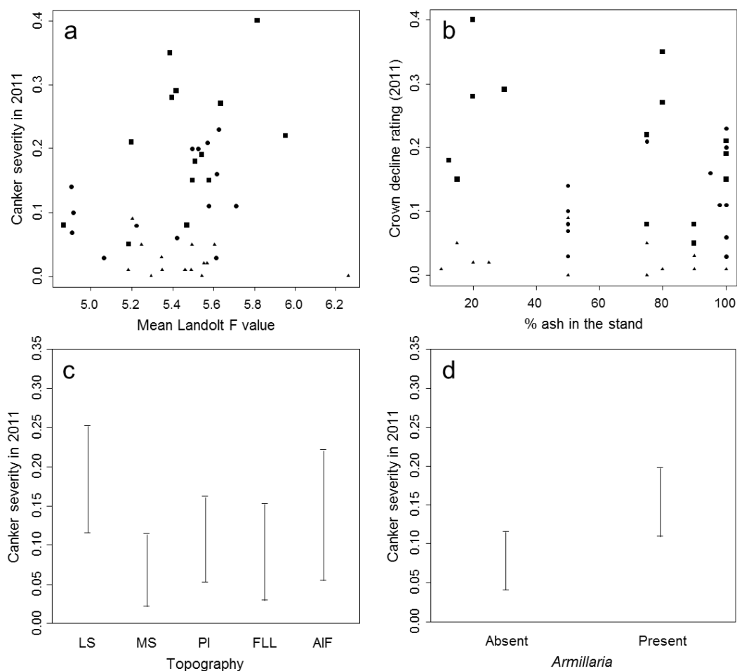
Figure 5. Influence of site and stand factor on the severity of collar lesions. a. Site humidity measured by the mean plot Landolt F value; b. % of ash in the stand; c. Topography: LS, lower slope, MS mid slope, PI, plateau, FLL, flat low land, AIF, Alluvial flooded site, d. Presence of Armillaria . ■, inside the H. fraxineus focus, i.e. spatially structured random effect of less than 0.11, ●, intermediate, i.e. spatially structured random effect of 0.11-0.16, closed ▲, outside the H. fraxineus focus, i.e. spatially structured random effect of more than 0.16 (see Fig. 1b). 0.11 and 0.16 represent the 0.33 and 0.66 percentile of the spatially structured random effect. Credibility intervals are shown on Fig. 5.c and d.
