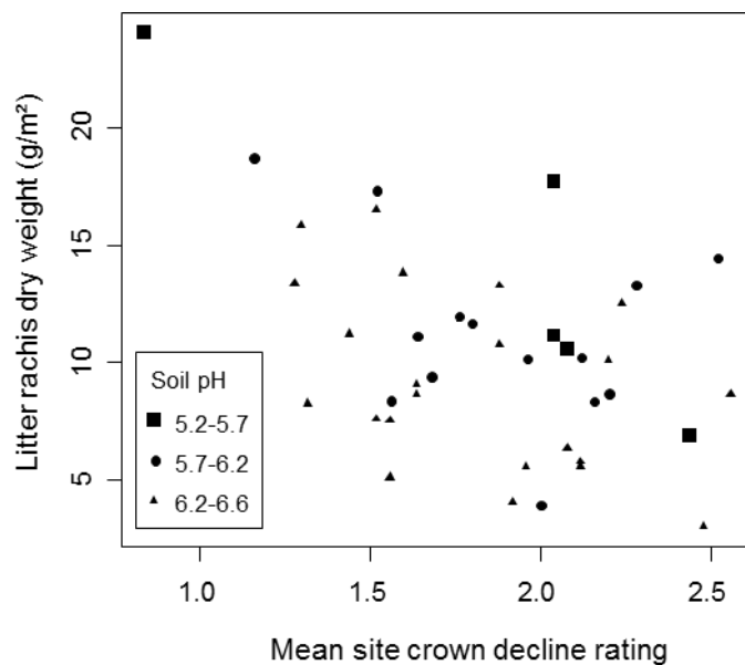
Figure 2. Ash rachis dry weight (ADW) in the soil litter.
