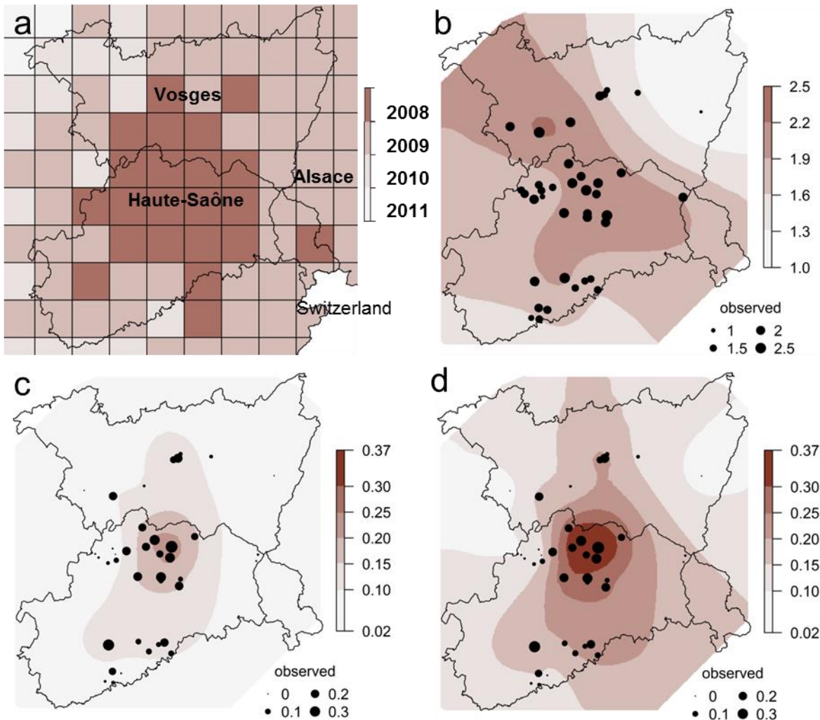
Figure 1. Spatial structure in disease severity; a; Year of first report of H. fraxineus by the health survey system (Département de la Santé des Forêts). b. Ash crown decline index in 2011. c, d. % collar girdled by the basal canker in 2011 (c) and 2012 (d). Heat maps shown in b, c, d are results of the model including only the spatially structured random effect and the intercept for respectively crown decline in 2011, collar girdling in 2011 and collar girdling in 2012 while the black circles (observed) represent the measured values for these variables.
