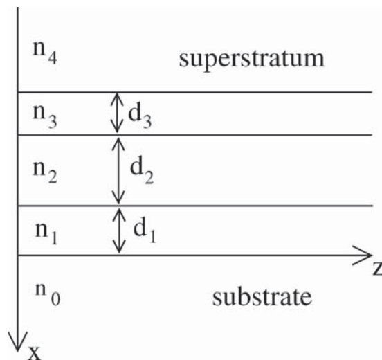
Figure 1. Three layer waveguide.
