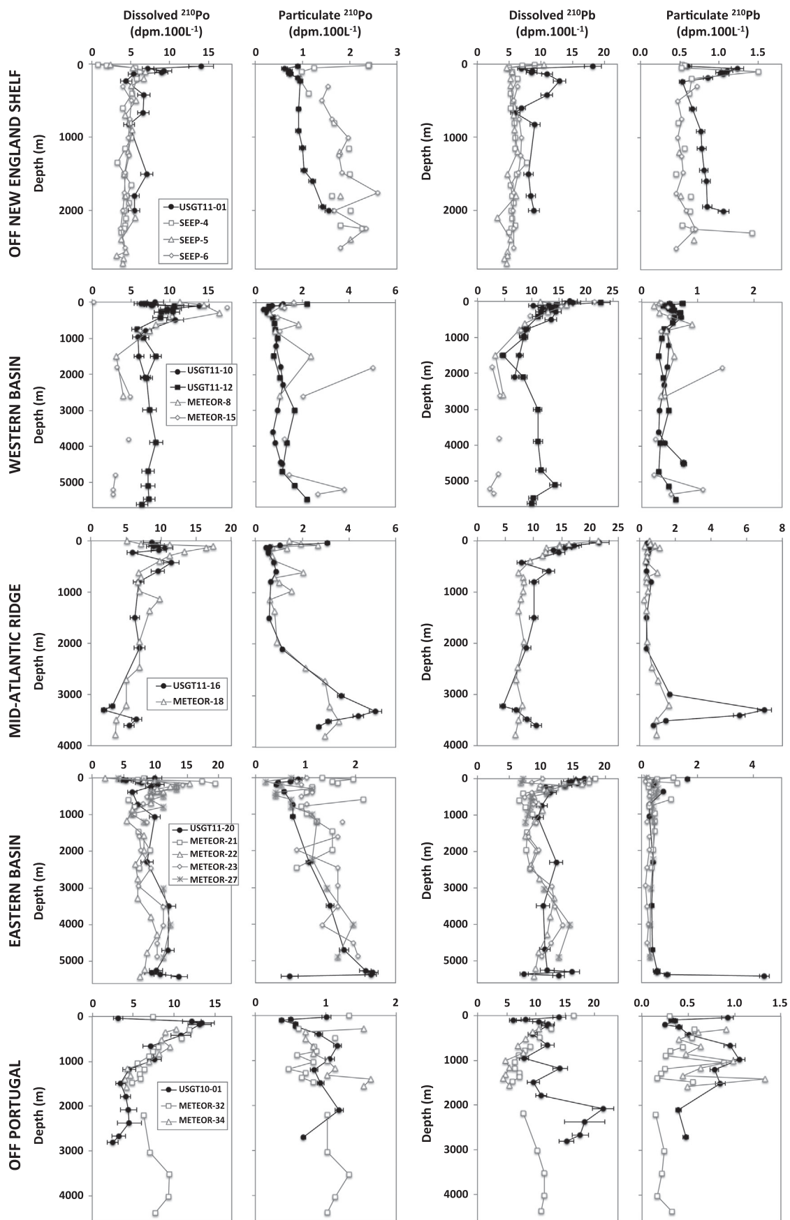
Fig. 8. Comparison of the dissolved and particulate 210 Po and 210 Pb activities obtained within the present study (USGT stations, in black) with those previously published by Bacon (1977) and Bacon et al. (1988) (METEOR and SEEP stations, respectively, in grey) in several sub-areas in the North Atlantic. The locations of the stations are reported in Fig. 1. USGT Particulate samples correspond to the sum of the small and large particulate fractions, excepted for the particulate samples deeper than 1000 m in station USGT10-01 for which large particulate data is not available.
