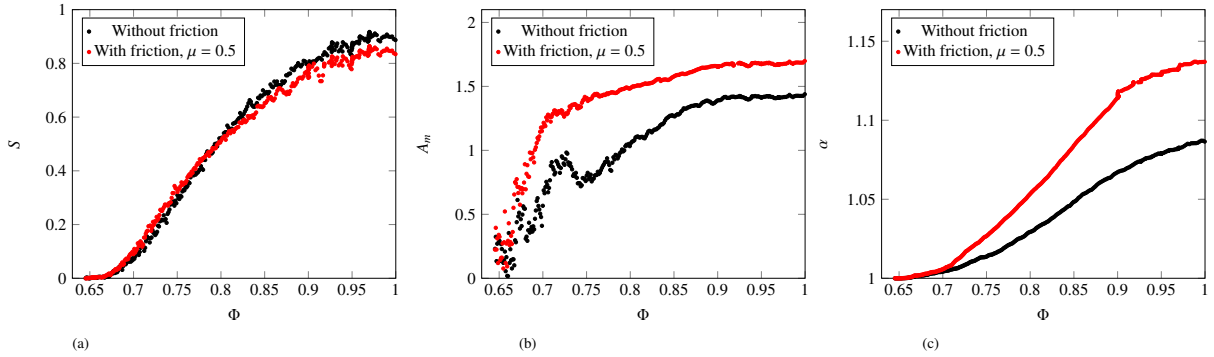
Fig. 2: Evolutions of mean contact specific surface S , mean orientation anisotropy A_m and mean aspect ratio \alpha as a function of packing fraction \Phi .
