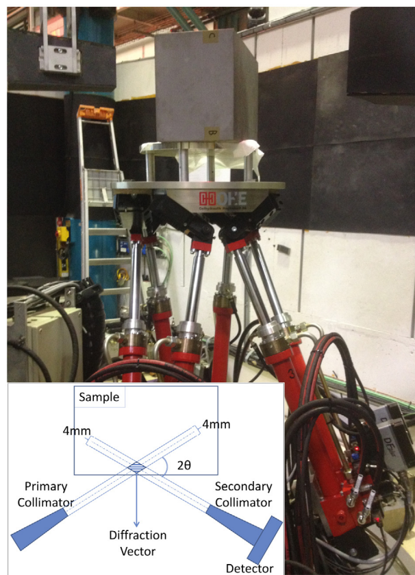
Fig. 3. Main parts of the SALSA instrument. The neutron beam arrives on the sample through the primary collimator (on the left). The sample is located on top of a hexapod and can be rotated and translated around multiple axes. The diffraction volume is defined by the second collimator (on the right-hand side of the image) which directs the incoming beam to the detector (not shown). Inset: Projection of the diffraction volume (shaded area) on the horizontal plane, defined by the two collimators.
