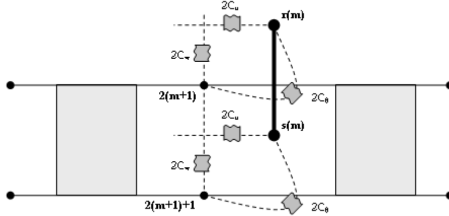
Fig. 5 A rigid body with the springs between the nodes 2(m+1) and 2(m+1)+1 simulating the fastener m .
