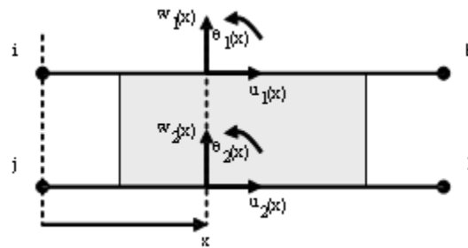
Fig. 3 Displacements in the “Bonded Beams” element.
