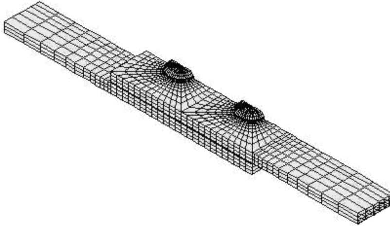
Fig 17 Finite Element model of the hybrid joint in single-lap configuration.
