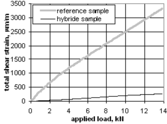
Fig. 16 Total shear strain measured from experimental tests.
