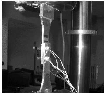
Fig. 15 Experimental set-up.
