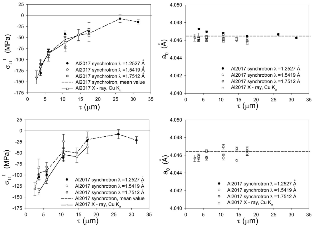
Fig. 5. The depth-dependent profiles of stress ( \sigma_{ii}^I ) and a_0 lattice parameter vs. penetration depth \tau for the polished (type II) sample. In the analysis the peak positions were determined by pseudo-Voigt function fitting (a) and using the centre of gravity method (b). The results for different wavelengths of synchrotron radiation and for Cu K_\alpha radiation are compared.
