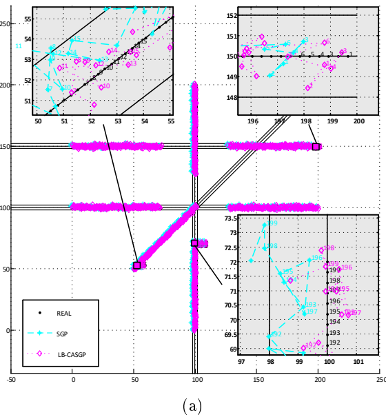
Figure 9: Trajectory and zoomed trajectory followed by each vehicle: (a) Simulation - vehicle 2 trajectory in the bottom-right zoom subplot; vehicle 6 trajectory in the top-right zoom subplot and vehicle 7 trajectory in the top-left zoom subplot (b) Real Experiments
