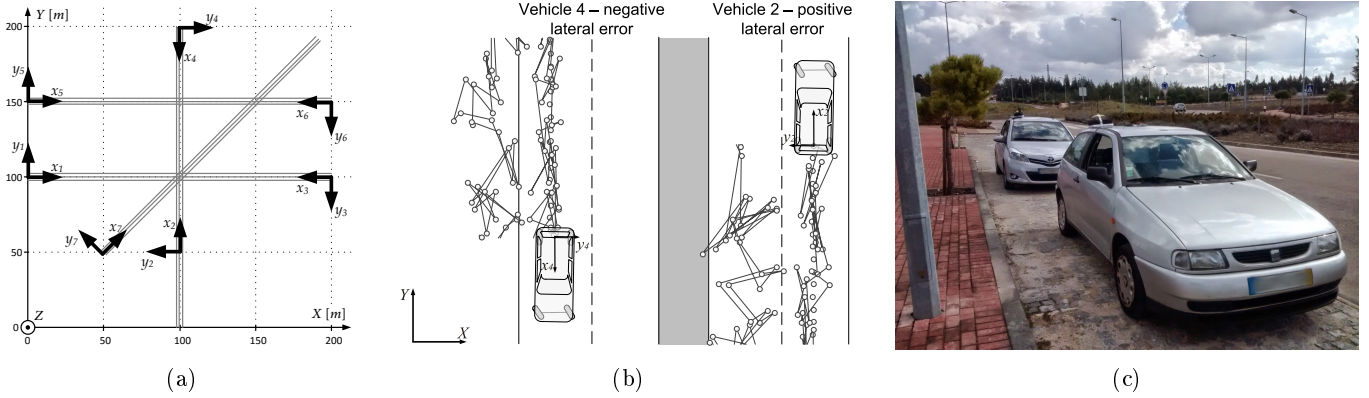
Figure 4: Setup: (a) Simulation environment - 7 vehicles simulated road network with starting vehicle positions and headings, vehicle x -axis and y -axis represent along-track and cross-track directions respectively; (b) Simulation - Zoomed trajectory and position estimation for vehicles 2 and 4. Vehicles 2 and 4 travel in a road lane parallel to the Y -axis local coordinates system \Sigma . Vehicle 2 is rotated by \pi/2 with respect to \Sigma . Vehicle 4 is rotated by 3\pi/2 with respect to \Sigma . The two vehicle's y -axis have opposite directions, leading to a positive lateral error for vehicle 2 and a negative lateral error for vehicle 4 in each vehicle local frame. This satellite constellation configuration generates an error with the major axis along the negative direction of the \Sigma X -axis; (c) Real Experiment - instrumented vehicles used in the tests;
