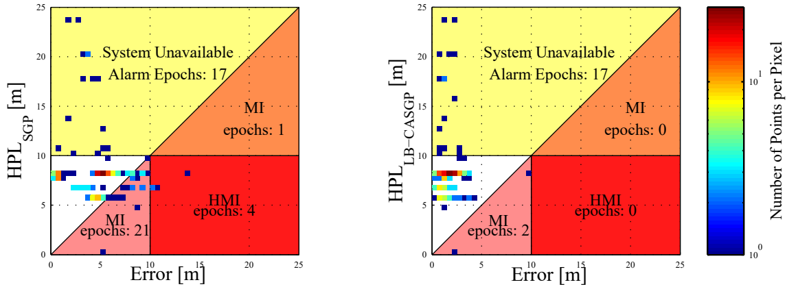
Figure 10: Real Experiments - HPL Stanford diagram: misleading information (MI), hazardously misleading information (HMI)
