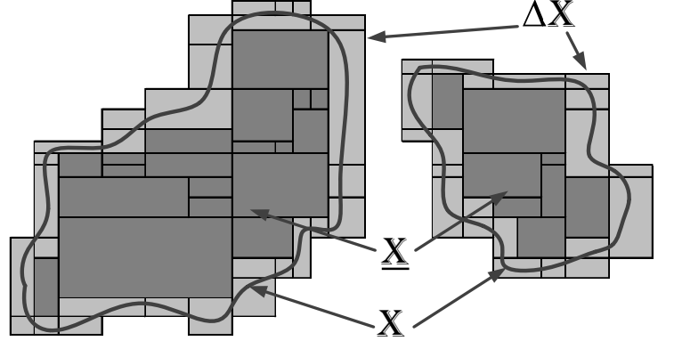
Figure 2: Compact set \mathbb{X} : bracketed between an inner subpaving \underline{\mathbb{X}} and an outer subpaving \overline{\mathbb{X}} , where \overline{\mathbb{X}} is given by \overline{\mathbb{X}} = \underline{\mathbb{X}} + \Delta\mathbb{X} .
