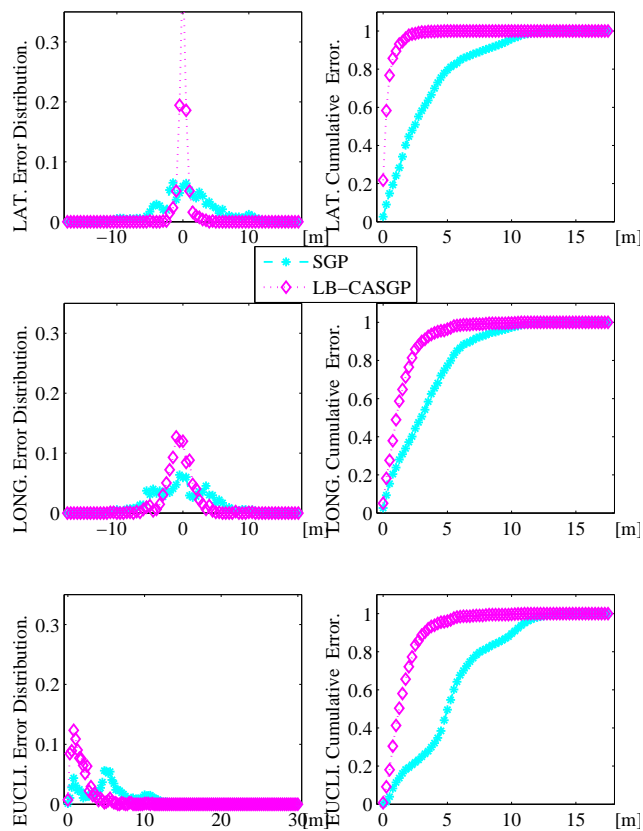
Figure 8: Real Experiments - All vehicles positioning errors, lateral (top), longitudinal (center) and 2D euclidean (bottom), using SGP and LB-CASGP estimation: (a) normalized positioning errors distribution. (b) cumulative distribution functions.
