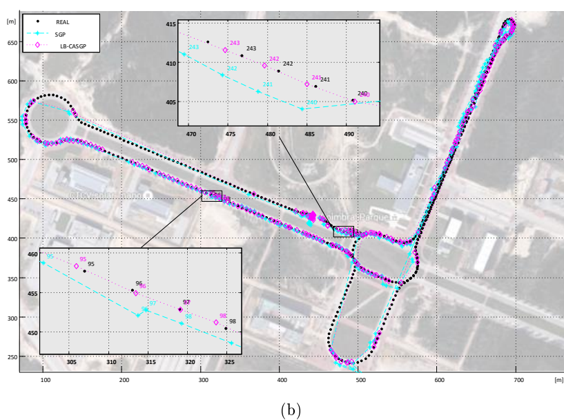
Figure 9: Trajectory and zoomed trajectory followed by each vehicle: (a) Simulation - vehicle 2 trajectory in the bottom-right zoom subplot; vehicle 6 trajectory in the top-right zoom subplot and vehicle 7 trajectory in the top-left zoom subplot (b) Real Experiments
