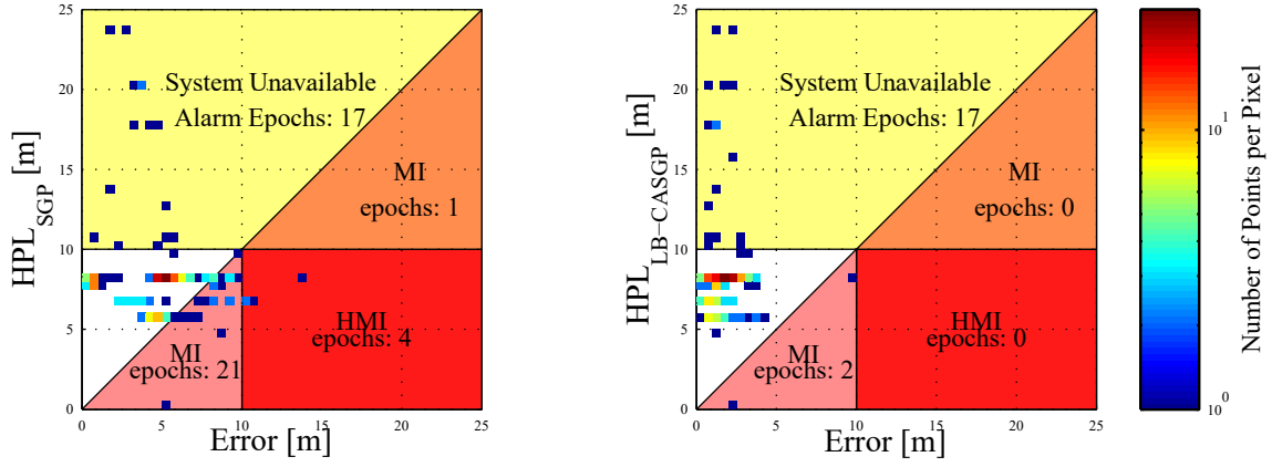
Figure 10: Real Experiments - HPL Stanford diagram: misleading information (MI), hazarously misleading information (HMI)
