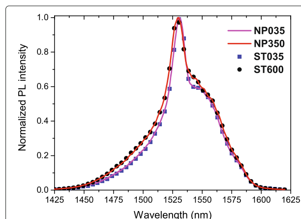
Fig. 2 Room temperature normalized PL spectra
