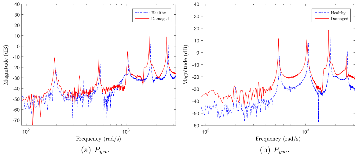
Fig. 9. Frequency response comparison between healthy and damaged structures.
