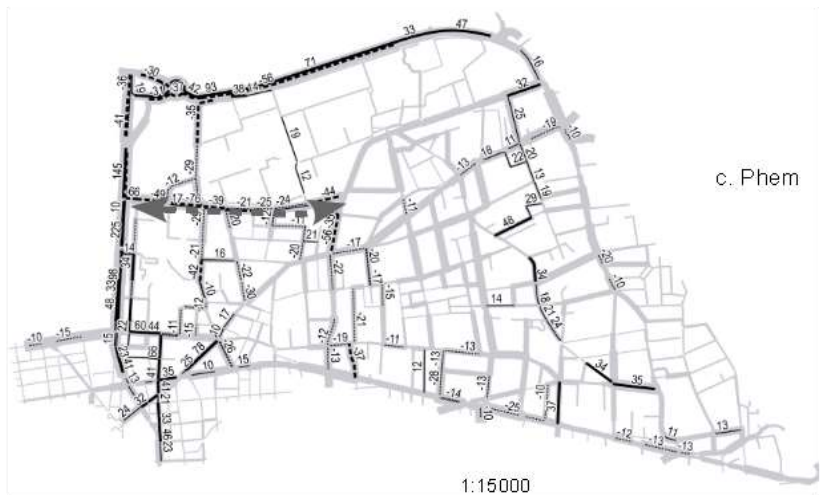
Figure 3: impact of the O11nov scenario on the estimated NOx emissions. NOx emissions of the reference scenario is figured in lighth grey, major differences of O11nov to the reference in dark. More explanations of method in the text.
