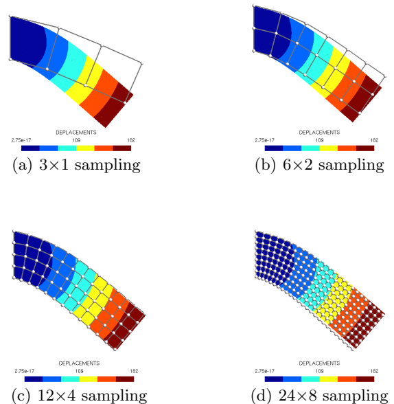
Fig. 12 Deflection experiment: the reference FEM solution (in color gradation) with superimposition of various simulations performed for different mesh resolutions).
