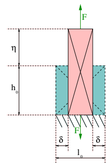
Fig. 2 The bar of dimension l_0 \times h_0 is elongated by a force \mathbf{F} , generating a stretch \eta and a compression of range 2\delta at equilibrium.
