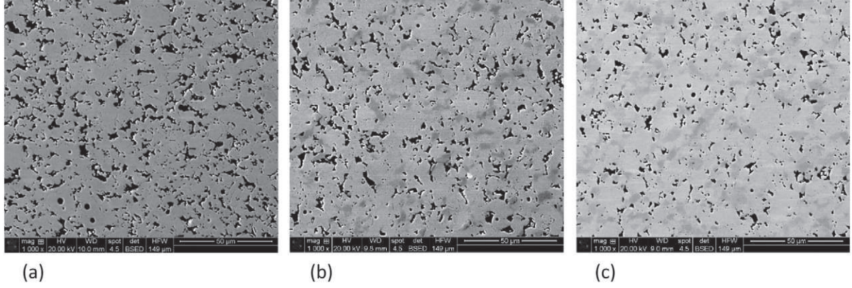
Fig. 3. SEM images of the specimen surfaces for pure YSZ matrix (a), YSZ and 10 vol.% MoSi 2 (b) and YSZ with 20 vol.% MoSi 2 (c).
