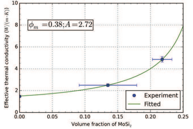
Fig. 8. Thermal conductivity of composites consisting of MoSi 2 spheres in an YSZ matrix. The solid line reflects theoretical predictions using Eqs. (3)–(6). Dots show experimental values measured at room temperature for actual volume fraction of MoSi 2 particles, as stated in Table 1.
