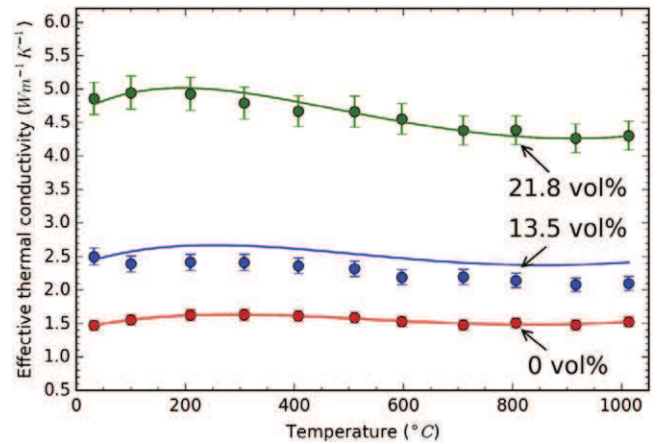
Fig. 9. Thermal conductivity of composites consisting of MoSi 2 spheres in an YSZ matrix. Dots show experimental data fitted into the Nielsen model (solid line) according to the actual volume fraction of MoSi 2 particles [26].
