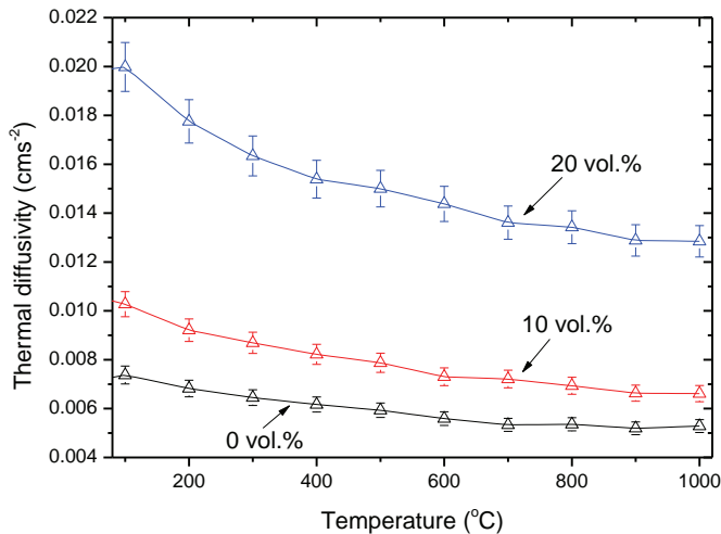
Fig. 5. Thermal diffusivity of the YSZ/MoSi 2 as a function of temperature.
