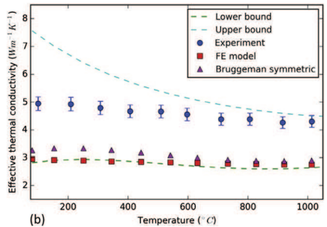
Fig. 7. Comparison of the temperature dependent thermal conductivity based on FE and the Bruggeman model solution for composite samples with 10 vol.% (a) and 20 vol.% MoSi 2 filler (b). Dashed lines show lower and upper boundary regions for the asymmetric Bruggeman model.
