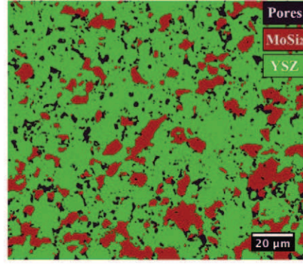
(b) Phase map
