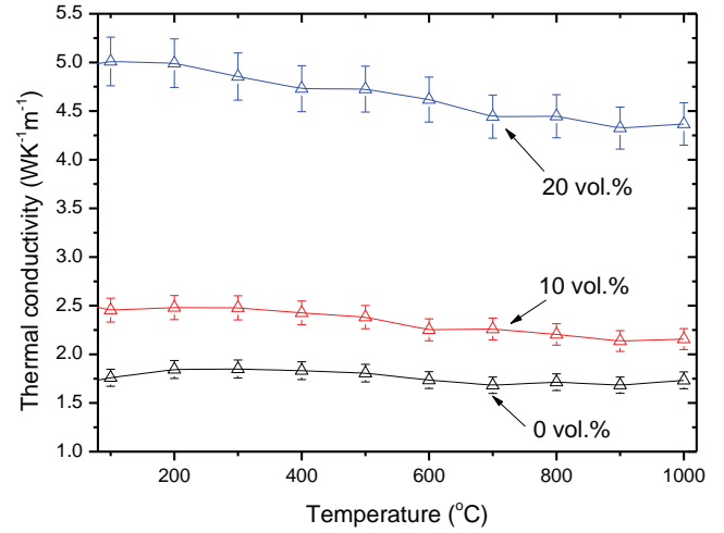
Fig. 6. Thermal conductivity of the YSZ/MoSi 2 as a function of temperature calculated using Eq. (1).
