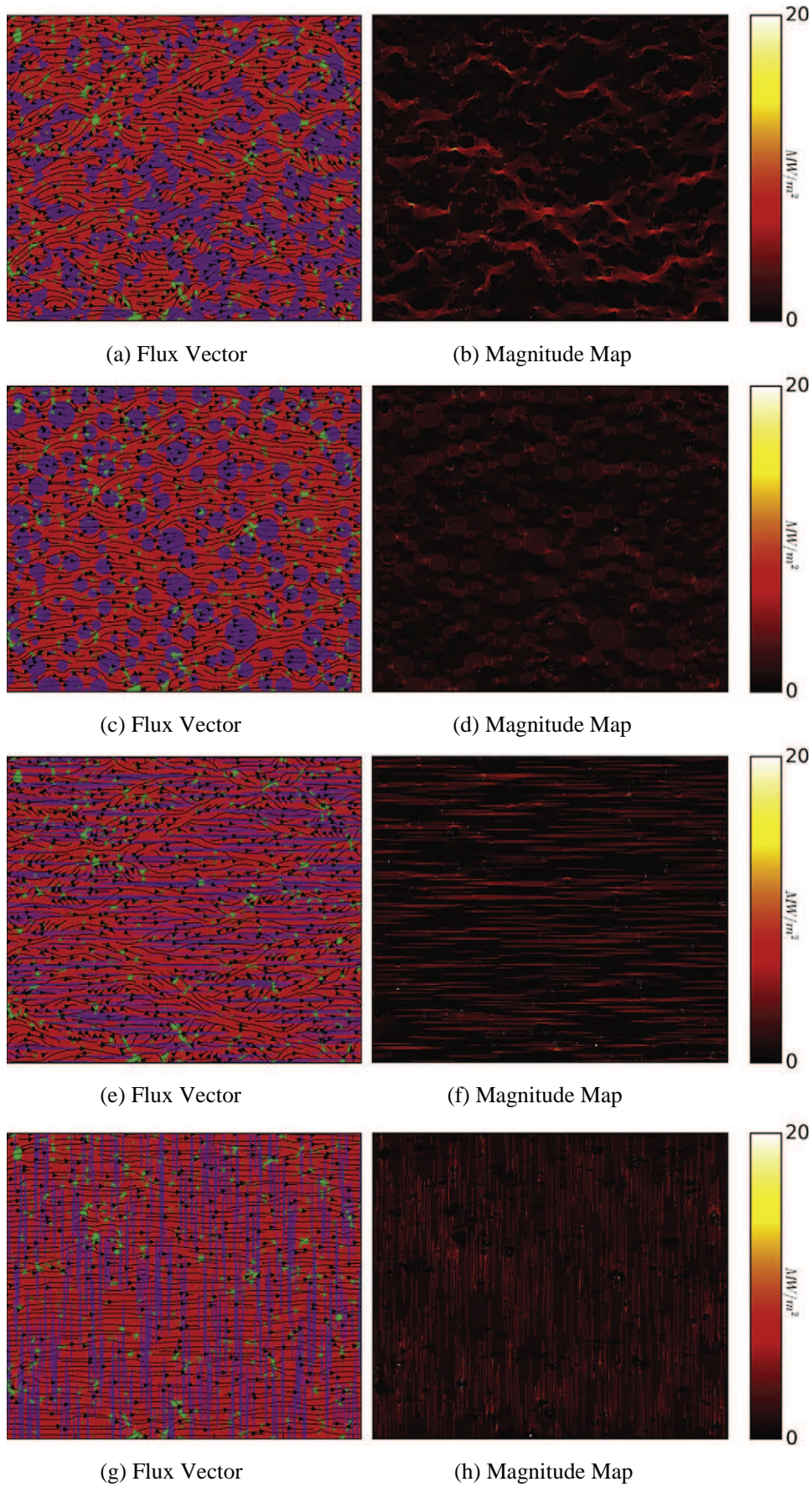
Fig. 12. Heat fluxes inside the ceramic composites with different MoSi 2 shapes: real microstructure, k_{eff} = 4.18 \text{ Wm}^{-1} \text{ K}^{-1} (a-b); a:c = 1:1 , k_{eff} = 3.38 \text{ Wm}^{-1} \text{ K}^{-1} (c-d); a:c = 32:1 , k_{eff} = 7.77 \text{ Wm}^{-1} \text{ K}^{-1} (e-f) and a:c = 1:32 , k_{eff} = 2.75 \text{ Wm}^{-1} \text{ K}^{-1} (g-h). The shape of MoSi 2 strongly affects the heat fluxes as they serve as channels for thermal flow.
