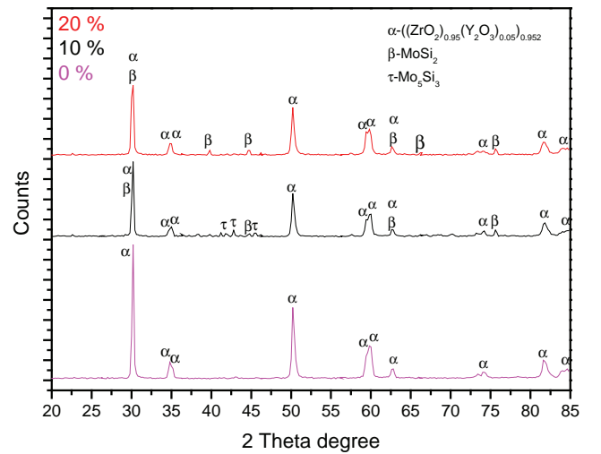
Fig. 4. XRD peak positions collected from SPS samples. Peaks have been assigned to different phases found from the analysis.
