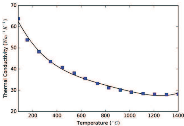
Fig. 2. Thermal conductivity of MoSi 2 as a function of temperature [11].
