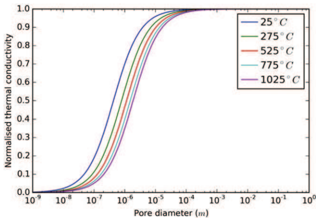
Fig. 10. Conductivity of Ar as a function of pore sizes at various temperatures according to Eq. (8).
