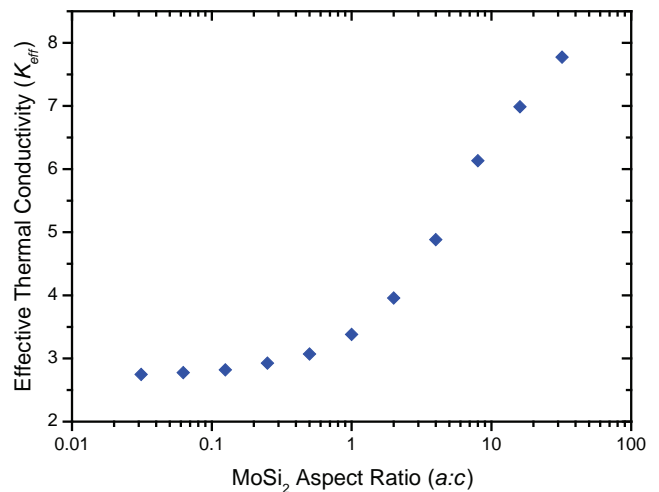
Fig. 11. Effective thermal conductivity values as a function of the \text{MoSi}_2 aspect ratio a:c calculated for modelled artificial microstructures.
