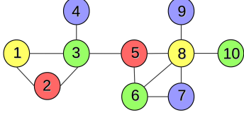
Fig. 6: Conflict graph for a ten-node network.
