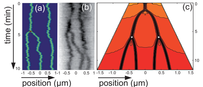
FIG. 2. (Color online) (a) Kymograph obtained from the model using an additional brownian force acting on ParBS: the model describes ParBS equilibrium, segregation and positioning. (b) Example of an experimental kymograph, obtained from 10 min. timelapse microscopy (frame every 10 sec.) of F-plasmids in E.coli , displaying a segregation event from two to three ParBS over the length of the nucleoid. (c) Theoretical kymograph obtained with growing cell (with an average over the stochastic noise). Trajectories are similar to experimental ones [5]. For details see SM.
