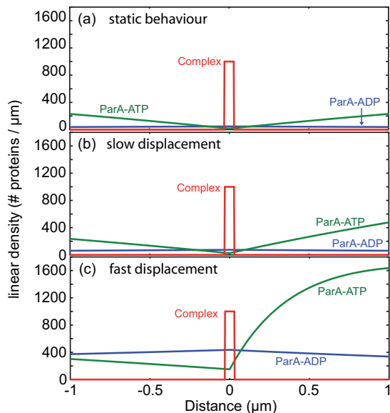
FIG. 3. (Color online) Density profile of ParA-slow v (green), ParA-fast u (blue) and ParBS (red). (a) \alpha < \alpha_c : positioning in the middle of the cell. (b) weak coupling \alpha_c \lesssim \alpha : ParBS moves as a TW and is "surfing" to the right on a protein wave. (c) strong coupling \alpha_c \ll \alpha : large asymmetry between the two sides of ParBS implying fast "surfing". See SM for details.
