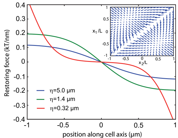
FIG. 1. (Color online) Proteophoresis force (Eq.(5)) for different values of the screening length \eta (variable k_1 ) with the other biological parameters fixed (see SM). The curve in blue is plotted using physiological values ( k_1 = 0.04 \text{ s}^{-1} ) and shows a marked restoring force gradient toward mid-cell positions: for \eta = 0.32, 1.4 and 5 \mu\text{m} , the force produces a parabolic potential well of depth \sim 0, 6 and 4 \text{ kT} , respectively, over a half-width of 0.25 \mu\text{m} (note the non-monotonic behavior with the equilibrium position restoring force vanishing for both zero and infinite k_1 , see SM). Inset: Proteophoresis force field in the phase space (x_1/L, x_2/L) of two partition complex positions.
